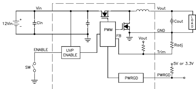
Figure 23: Block Diagram
