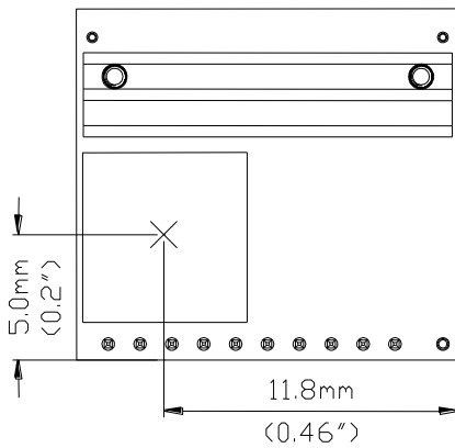
Figure 39: Temperature measurement location
