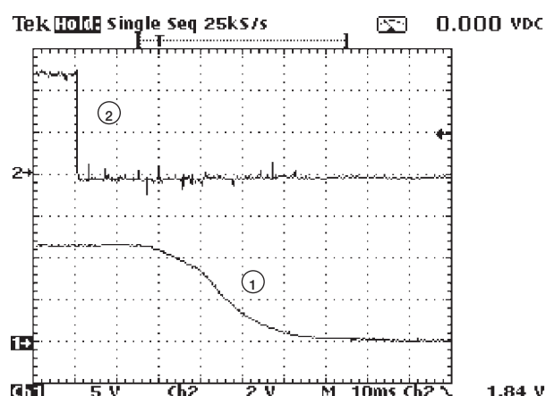
Figure 23 PF/DC OK signal 'V' V1 switch off full load
