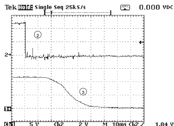
Figure 25 PF/DC OK signal 'V' V2 switch off full load
