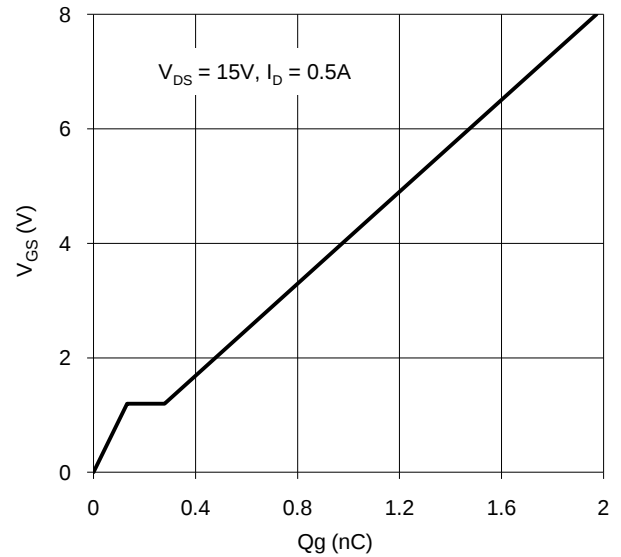
Figure 10. Gate Charge
