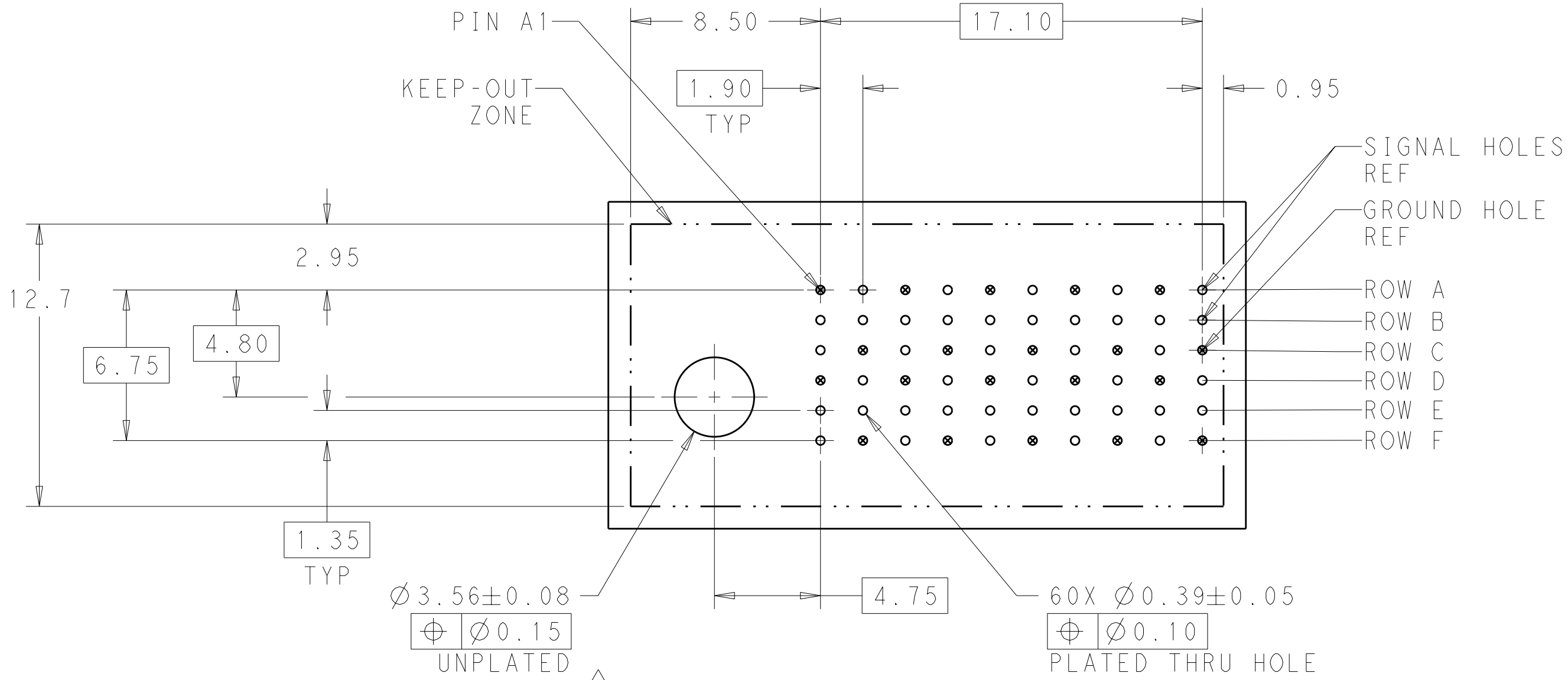
LEFT GUIDED BACKPLANE HOLE PATTERN (CONNECTOR SIDE)
