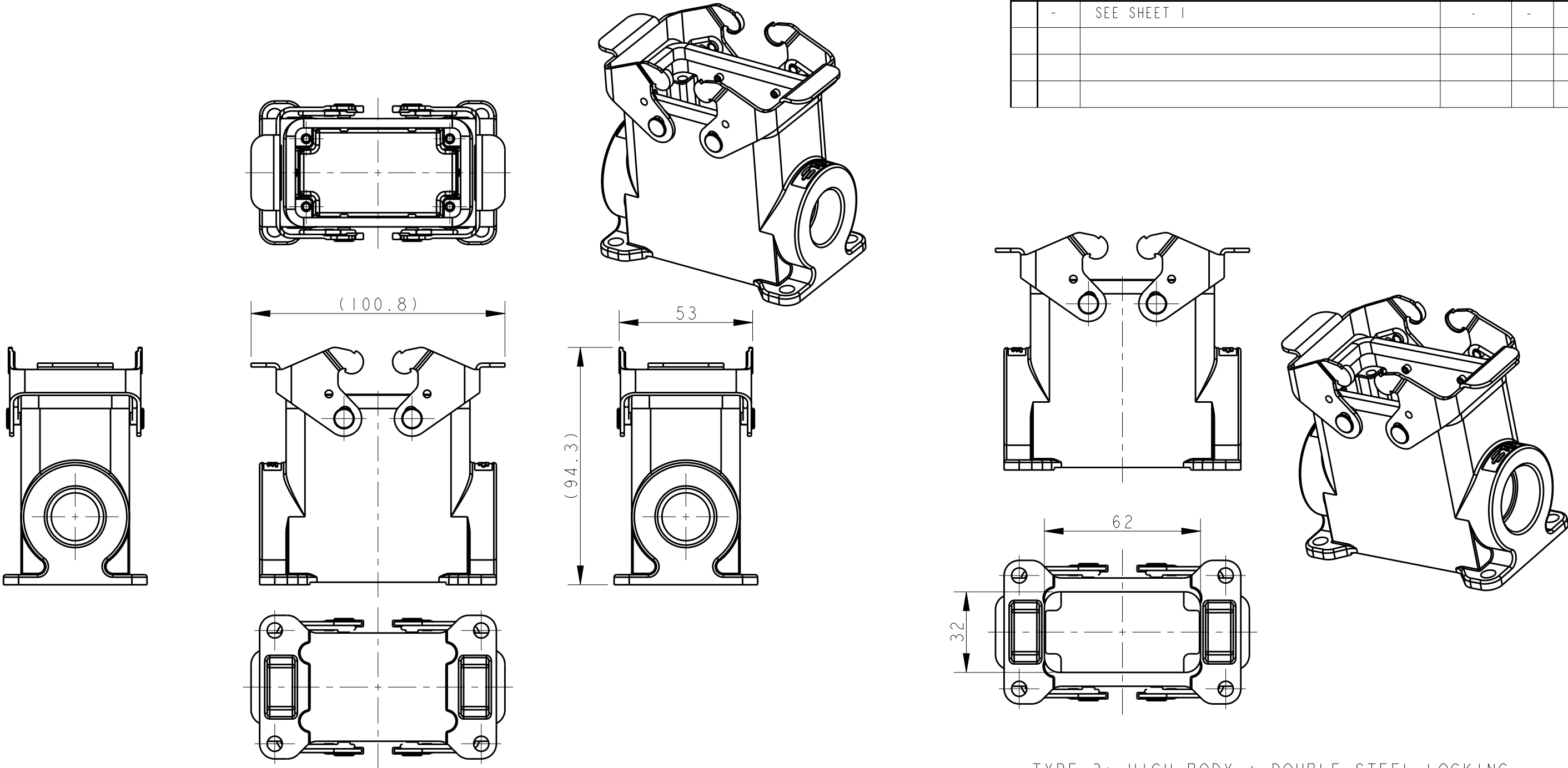
TYPE 3: HIGH BODY + DOUBLE STEEL LOCKING BOTTOM CUT OUT OTHER SPEC REFER TO TYPE 2
