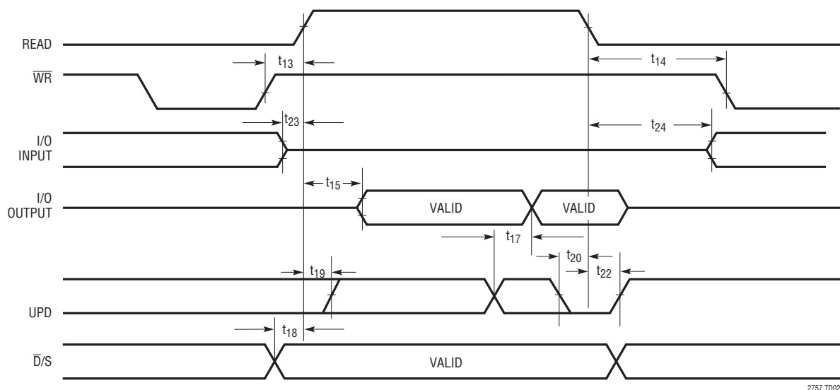
Readback Timing
