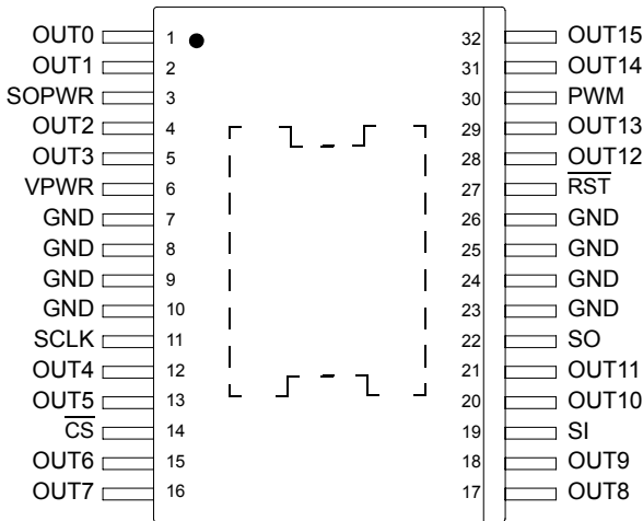
Figure 3. 33996 Pin Locations
