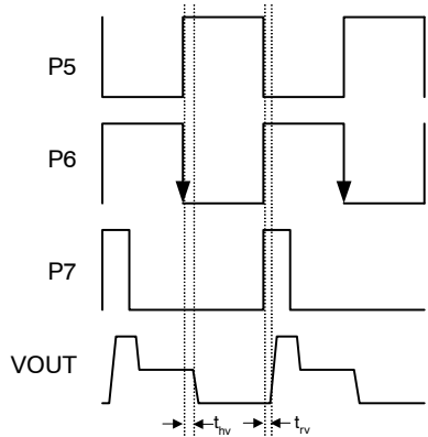
Figure 22. Pixel Timing Detail
