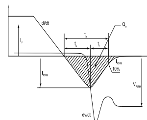
Figure 32: Diode reverse recovery waveform
