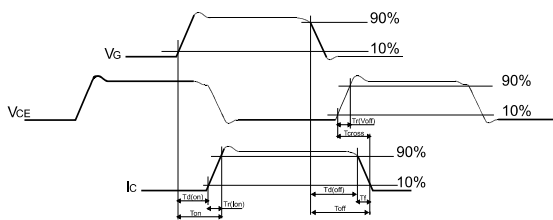
Figure 31: Switching waveform
