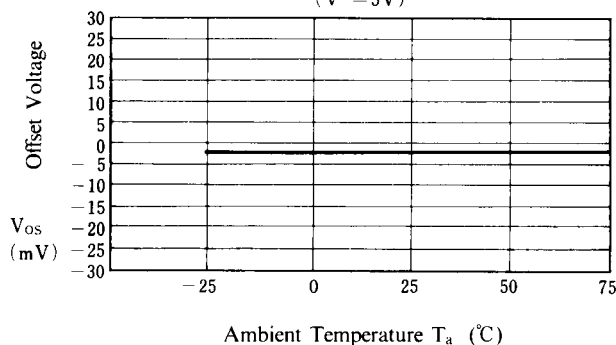
Offset Voltage vs. Ambient Temperature
