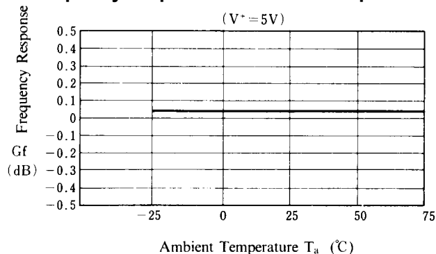
Frequency Response vs. Ambient Temperature
