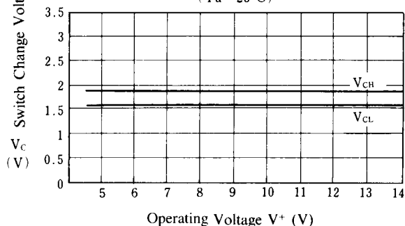
Switch Change Voltage vs. Operating Voltage
