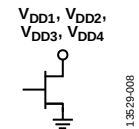
Figure 8. VDD1 to VDD4 Interface Schematic
