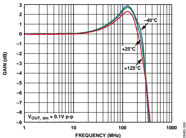
Figure 9. Small Signal Frequency Response for Various Temperatures (LFCSF)
