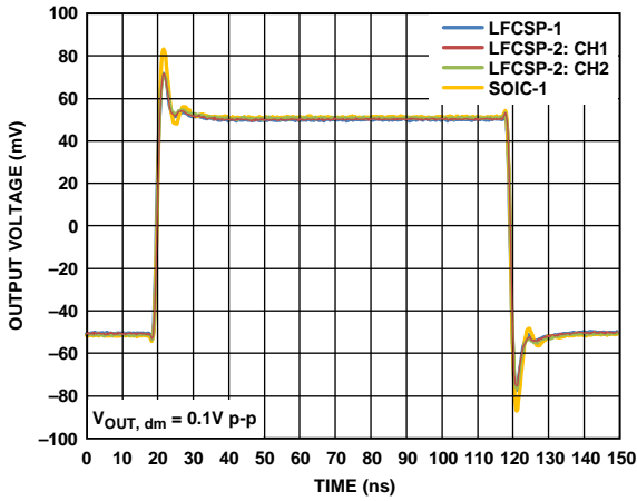
Figure 55. Small Signal Transient Response for Various Packages, C_L = 0\text{ pF}
