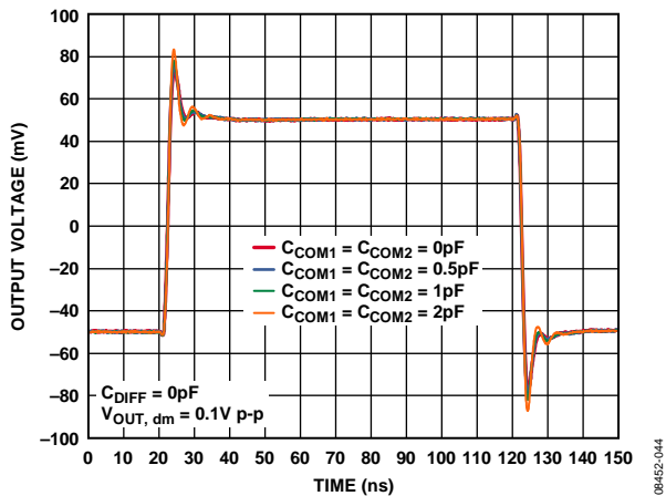
Figure 51. Small Signal Transient Response for Various Capacitive Loads (LFCS)
