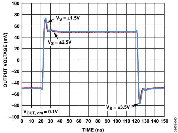
Figure 50. Small Signal Transient Response for Various Supplies (LFCS)
