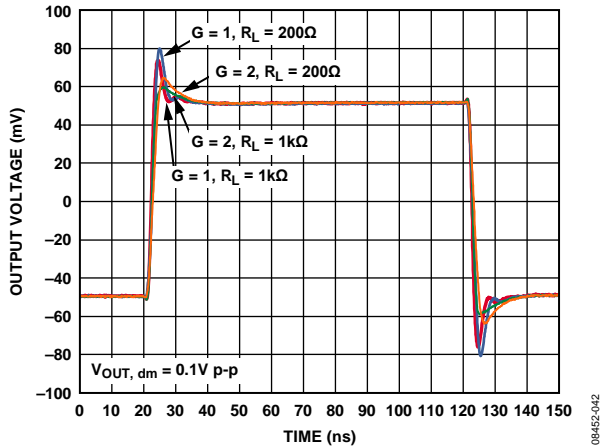
Figure 49. Small Signal Transient Response for Various Gains and Loads (LFCS)
