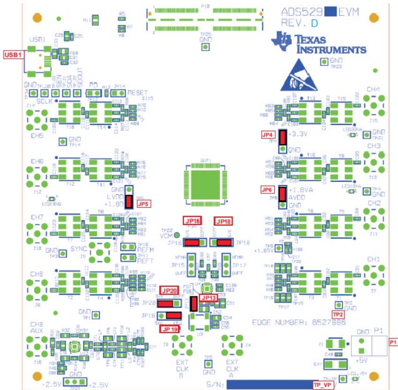
Figure 2. ADS5295EVM Basic Configuration
