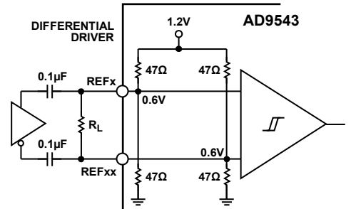
Figure 29. Differential AC-Coupled Mode ( R_1 = 100 \Omega Is Recommended, Except For HCSSL)
