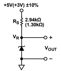
Figure 11. Typical Connection Diagram
