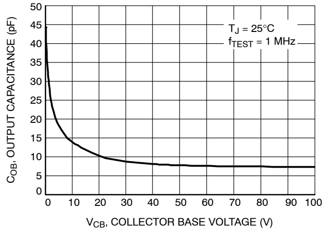
Figure 11. Output Capacitance
