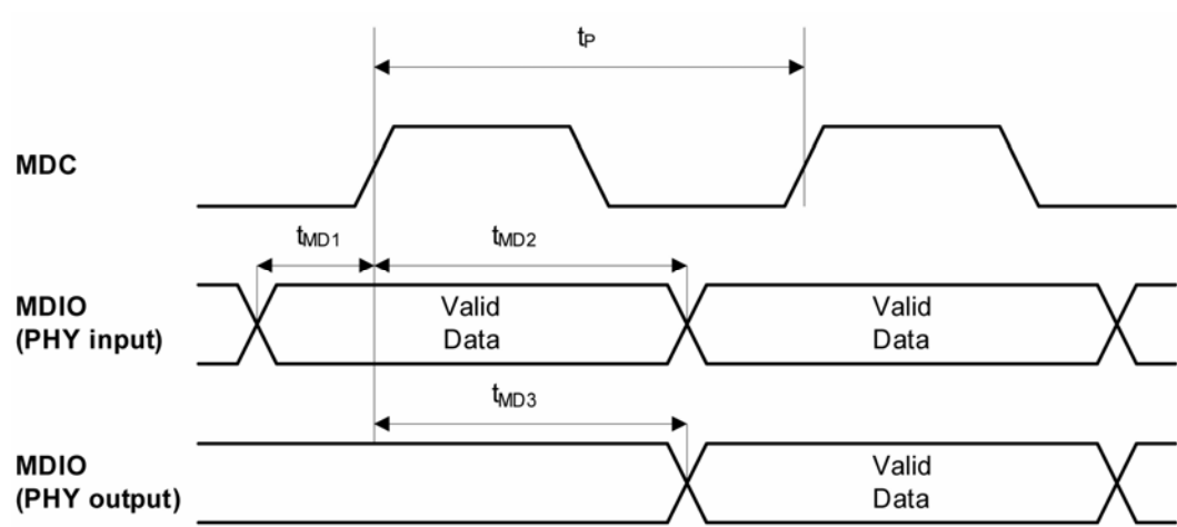
Figure 31. MDC/MDIO Timing
