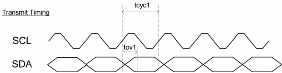
Figure 17. EEPROM Interface Output Timing Diagram
