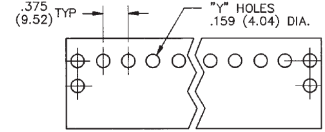
"Y" Terminal
