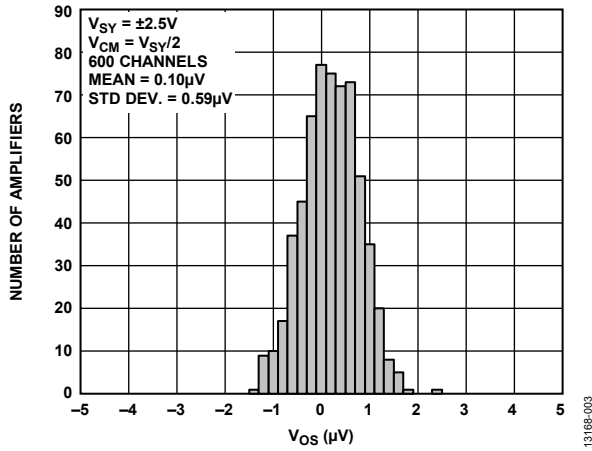
Figure 4. Input Offset Voltage Distribution, V_{SY} = \pm 2.5\text{ V}
