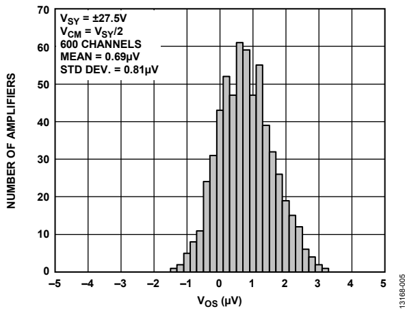
Figure 6. Input Offset Voltage Distribution, V_{SY} = \pm 27.5\text{ V}
