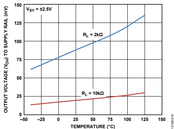
Figure 22. Output Voltage High ( V_{OH} ) to Supply Rail vs. Temperature, V_{SY} = \pm 2.5V
