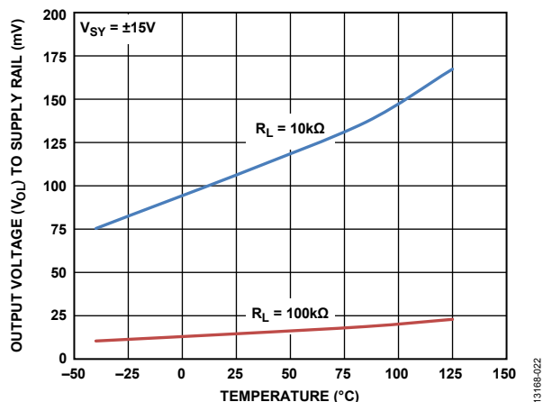
Figure 26. Output Voltage Low ( V_{OL} ) to Supply Rail vs. Temperature, V_{SY} = \pm 15V
