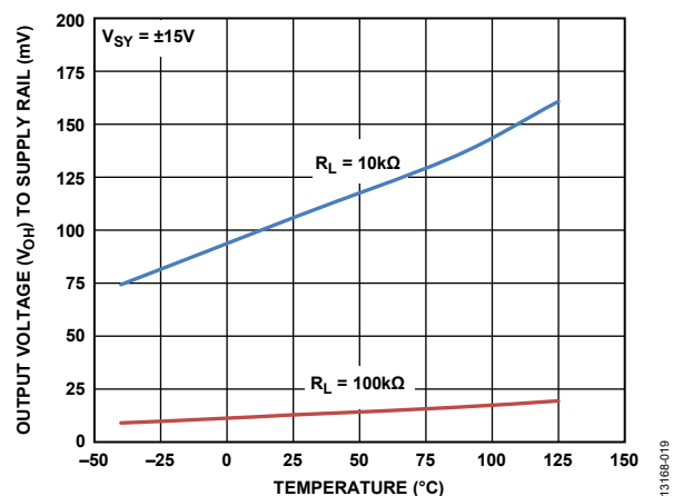
Figure 23. Output Voltage High ( V_{OH} ) to Supply Rail vs. Temperature, V_{SY} = \pm 15V
