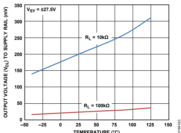
Figure 27. Output Voltage Low ( V_{OL} ) to Supply Rail vs. Temperature, V_{SY} = \pm 27.5V
