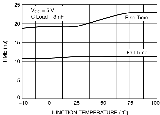
Figure 10. DRVL Rise and Fall Times vs. Temperature
