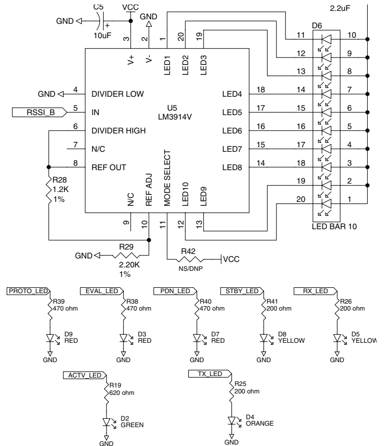
Figure 27: LEDs
