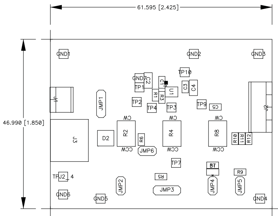
Figure 3. Top Assembly
