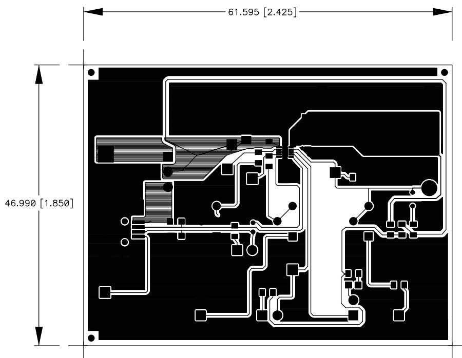
Figure 4. Top View
