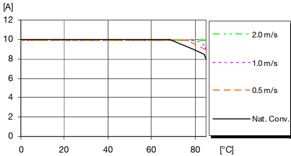
Available load current vs. ambient air temperature and airflow at V_I = 12.0 V, V_{OUT} = 1.8 V . See Thermal Consideration section.
