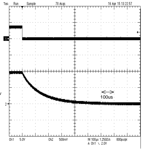
Figure 51. Shut down
