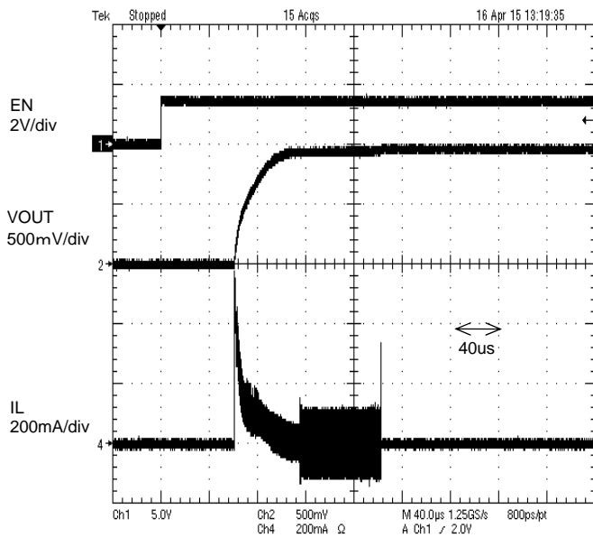
Figure 50. Start up
