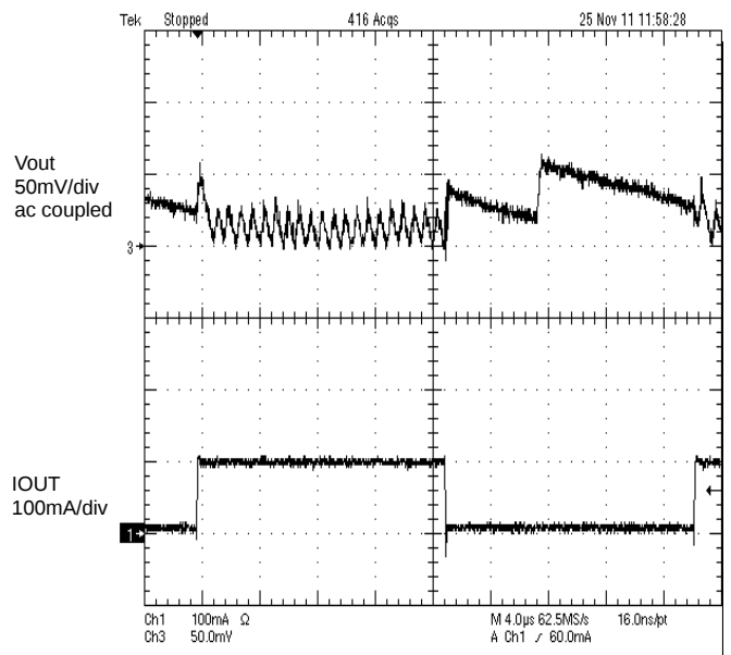
Figure 41. Load transient response 5mA to 100mA tr=tr=100ns , MODE : Low
