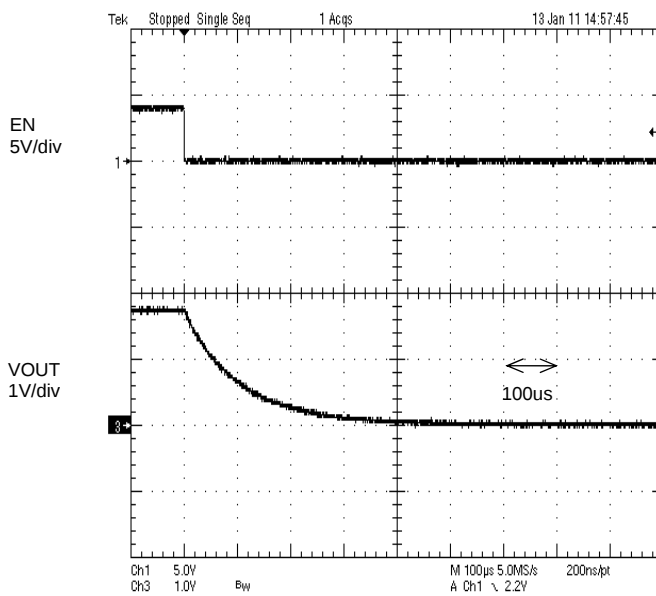
Figure 29. Shut down
