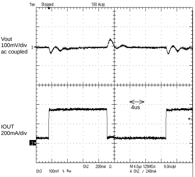
Figure 42. Load transient response 50mA to 350mA tr=tr=100ns , MODE : High
