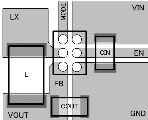
Figure 72. PCB layout
