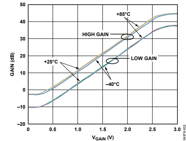
Figure 3. Gain vs. V_{GAIN} at Three Temperatures (See Figure 49)
