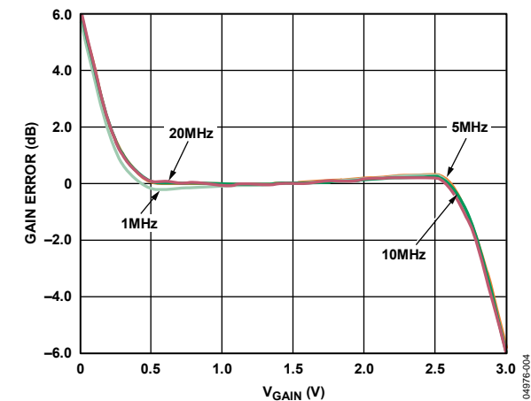
Figure 5. Gain Error vs. V_{GAIN} at Various Frequencies (See Figure 49)
