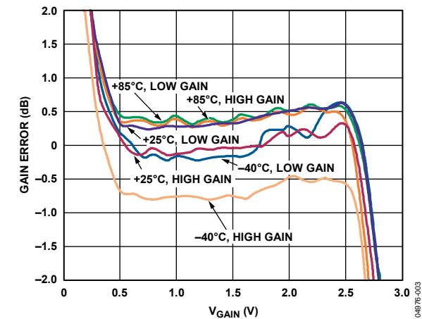
Figure 4. Gain Error vs. V_{GAIN} at Three Temperatures (See Figure 49)
