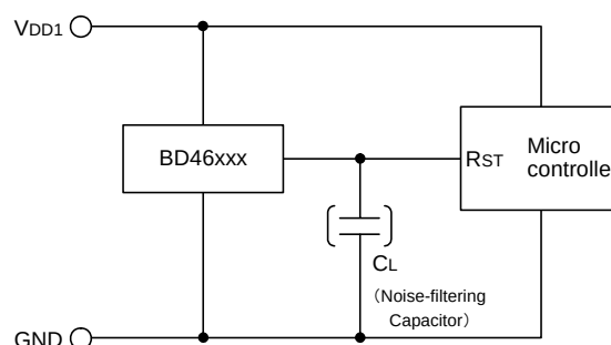
(CMOS Output Type) BD46xxx series
