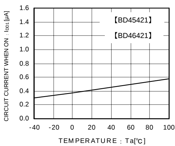
Fig.10 Circuit Current when ON ( V_{DET}-0.2V )
