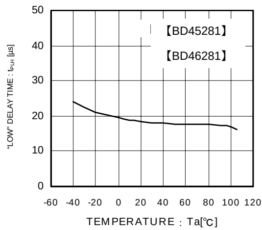
Fig.14 Output Delay Time "High" \rightarrow "Low"
