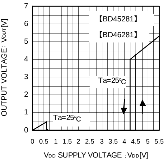
Fig.6 I/O Characteristics
