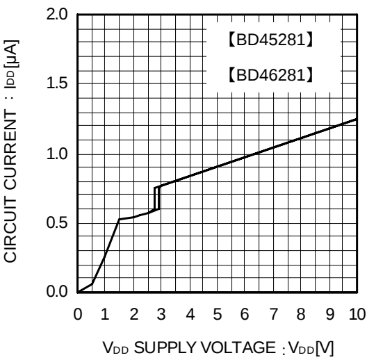
Fig.3 Circuit Current
