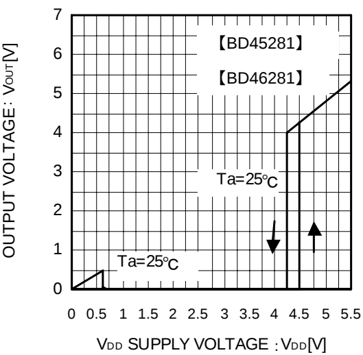
Fig.6 I/O Characteristics
