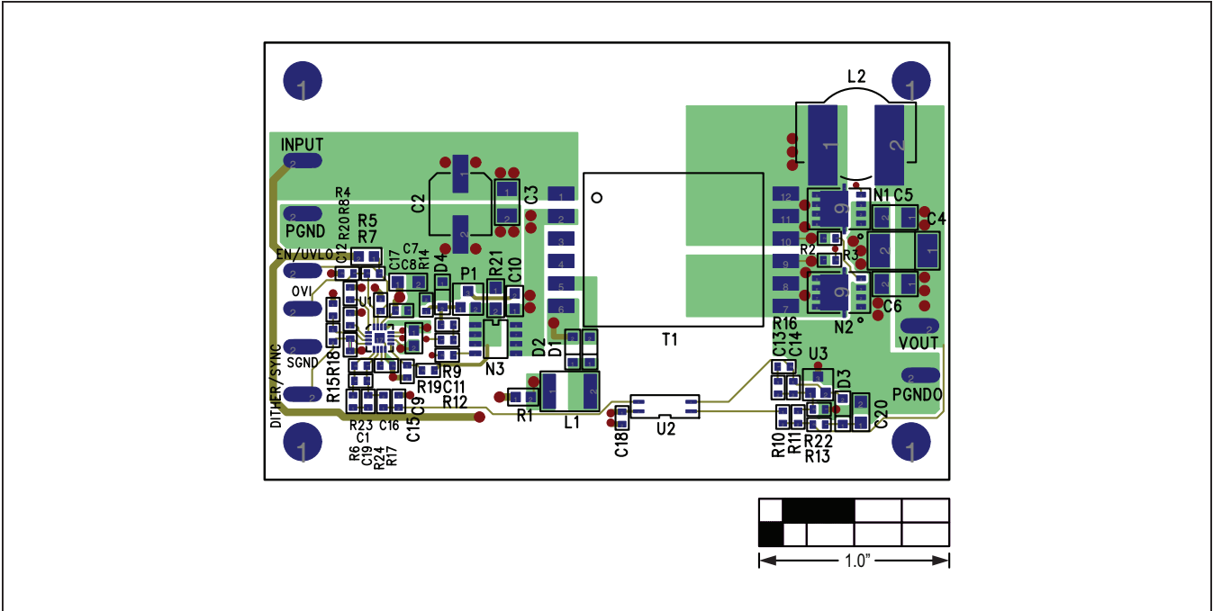
Figure 7. MAX17598 EV Kit PCB Layout—Component Side
