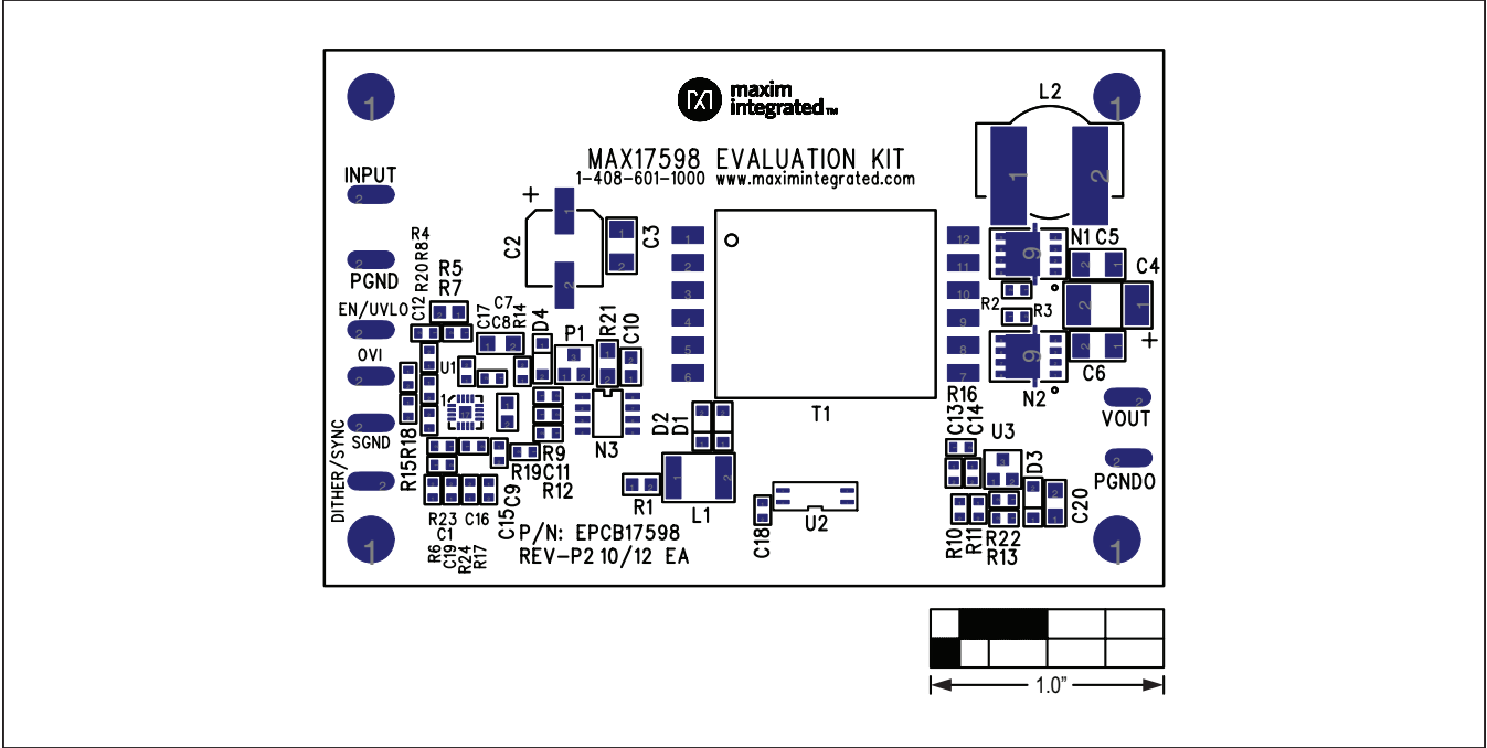
Figure 6. MAX17598 EV Kit Component Placement Guide—Component Side
