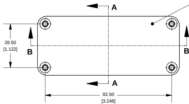
Top View of Assembly
