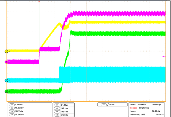
Figure 5: AC Input Voltage 85V ACIN , Full Load
