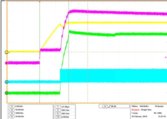
Figure 4: AC Input Voltage 85V ACIN , NO Load
