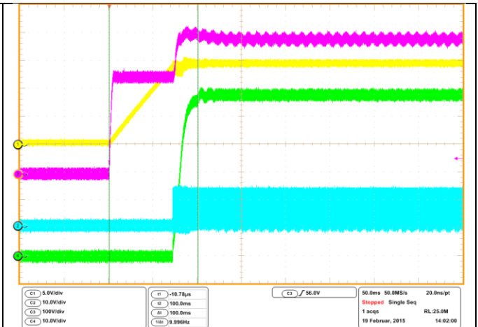
Figure 7: AC Input Voltage 230V ACIN , Full Load
