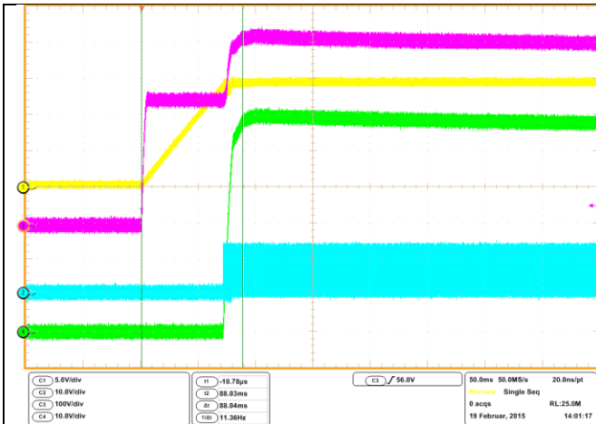
Figure 6: AC Input Voltage 230V ACIN , NO Load
