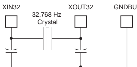
Figure 23-1. Typical Slow Clock Crystal Oscillator Connection
