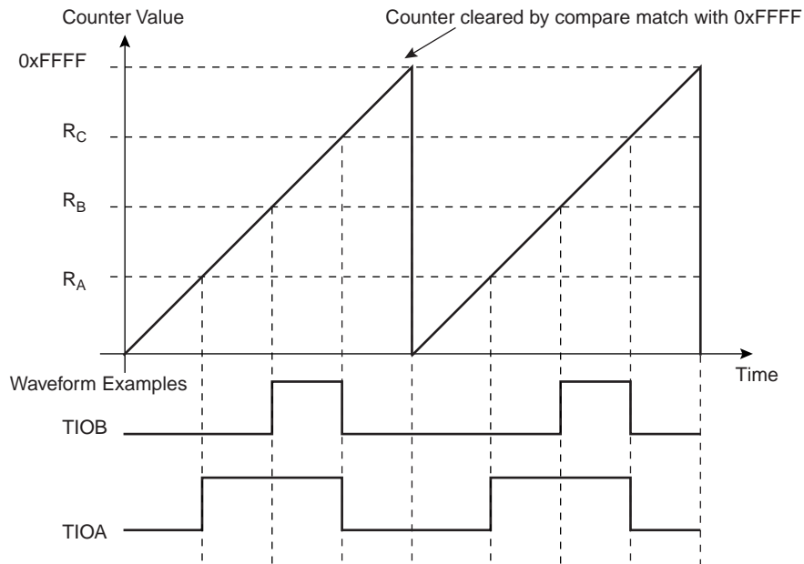
Figure 33-8. WAVSEL= 00 with trigger
