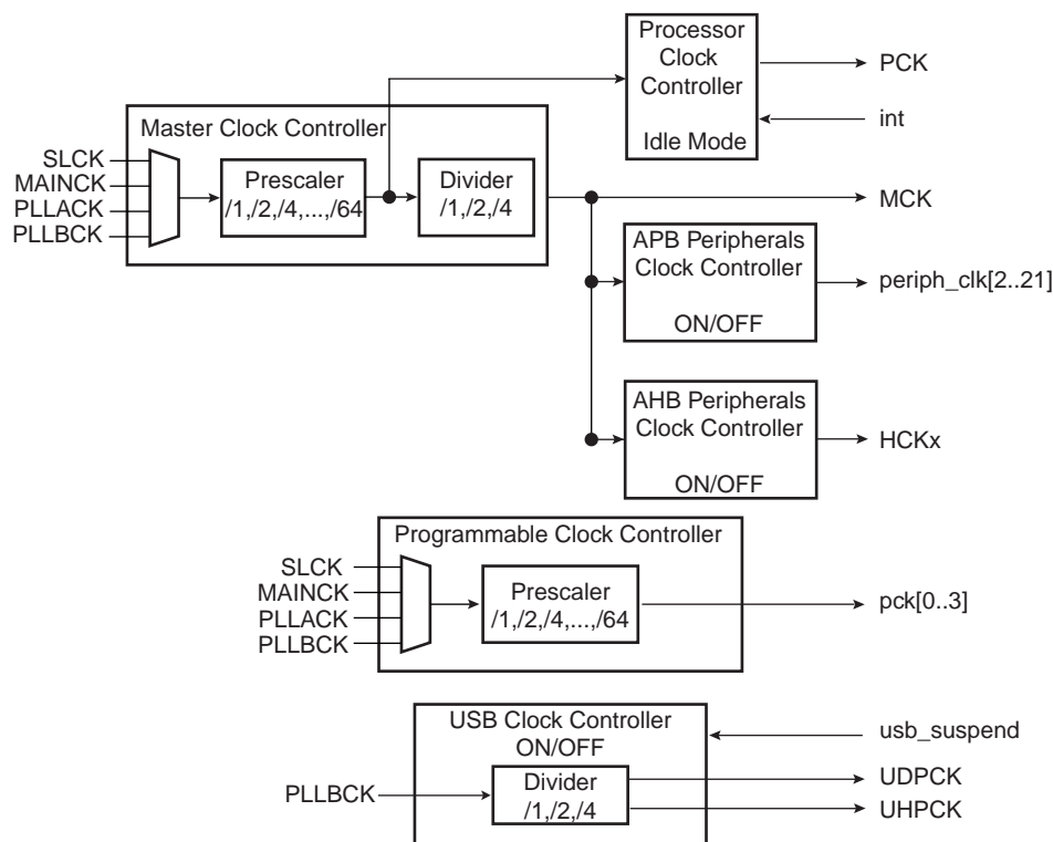
Figure 8-3. Power Management Controller Block Diagram
