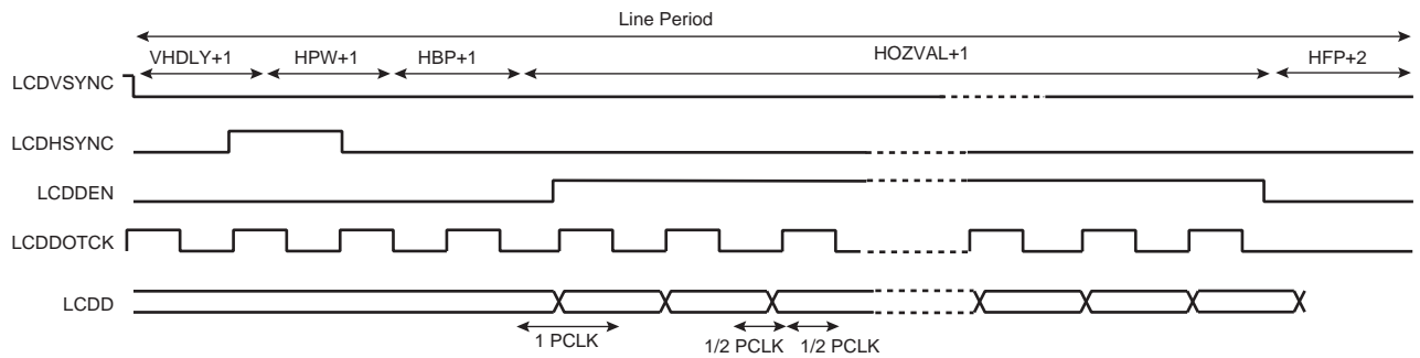
Figure 37-5. TFT Panel Timing (Line Expanded View), CLKMOD=1
