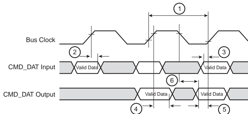
Figure 38-12. MCI Timing Diagram
