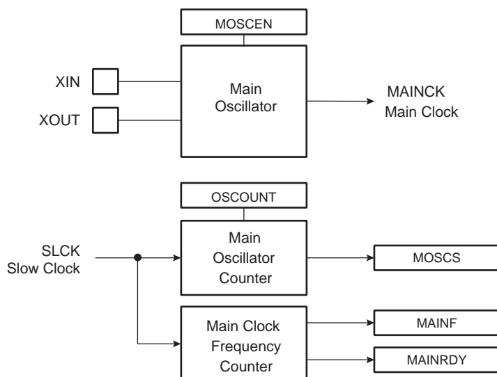
Figure 23-2. Main Oscillator Block Diagram
