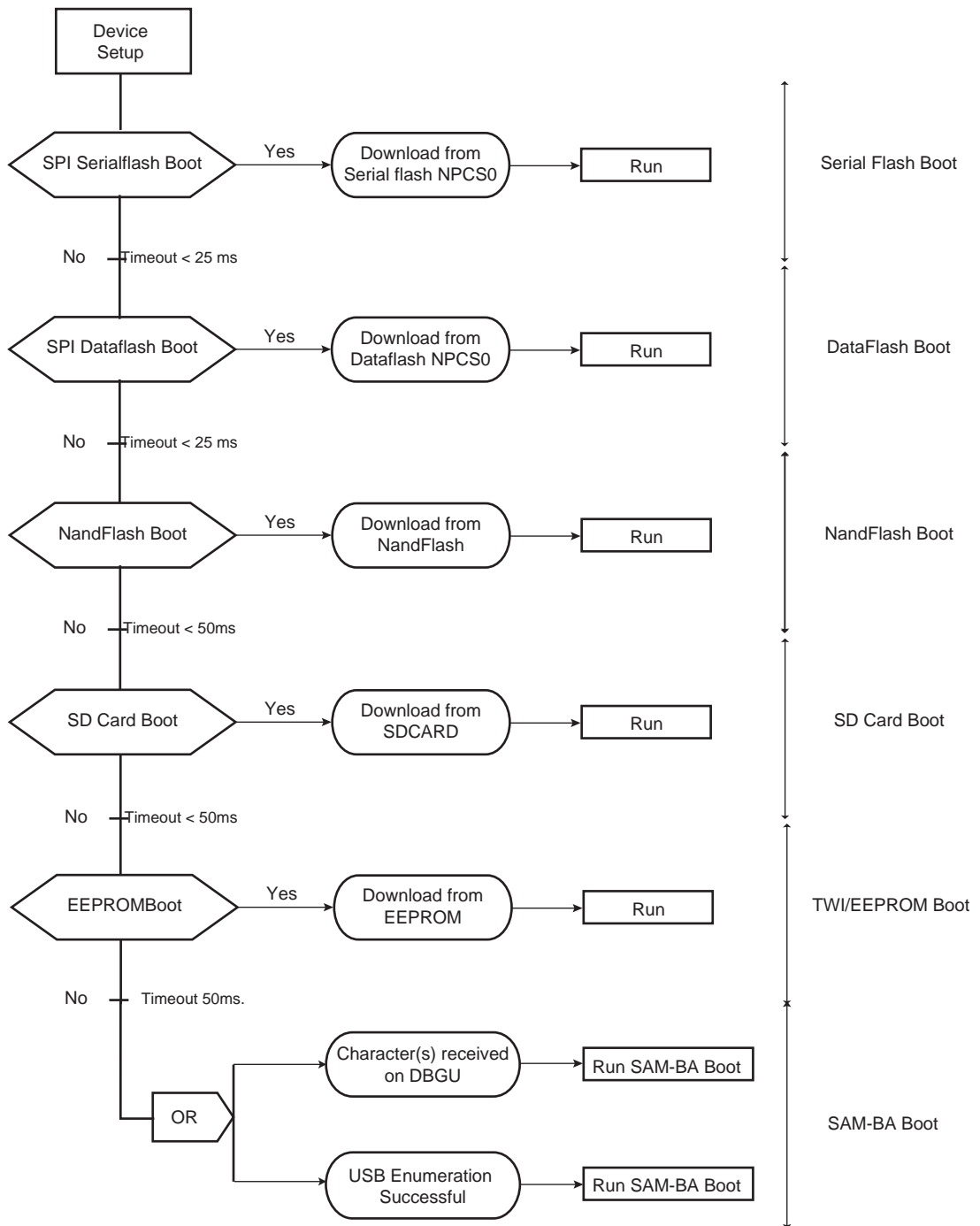
Figure 12-1. Boot Program Algorithm Flow Diagram
