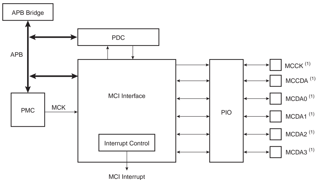
Figure 34-1. Block Diagram
