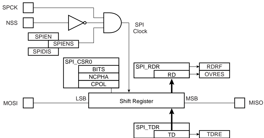
Figure 29-9. Slave Mode Functional Bloc Diagram
