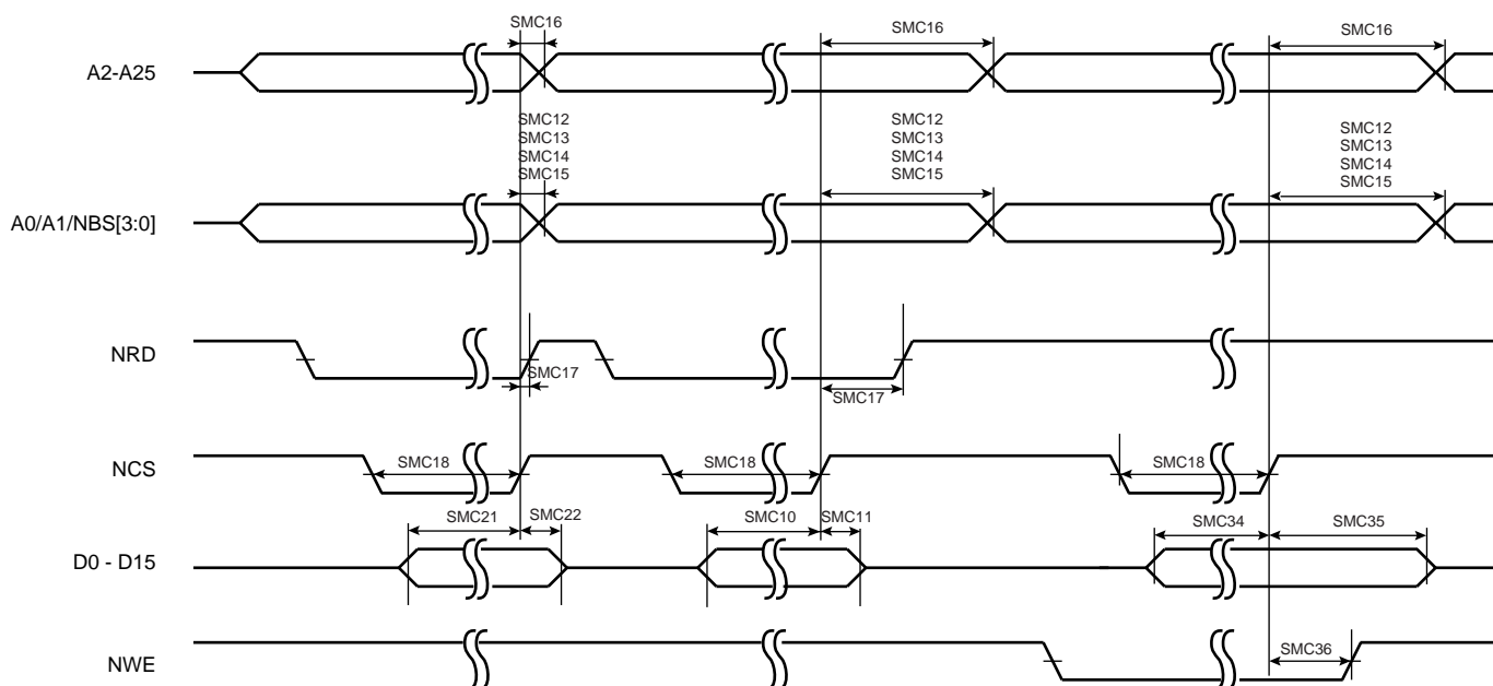
Figure 38-4. SMC NCS Controlled Access
