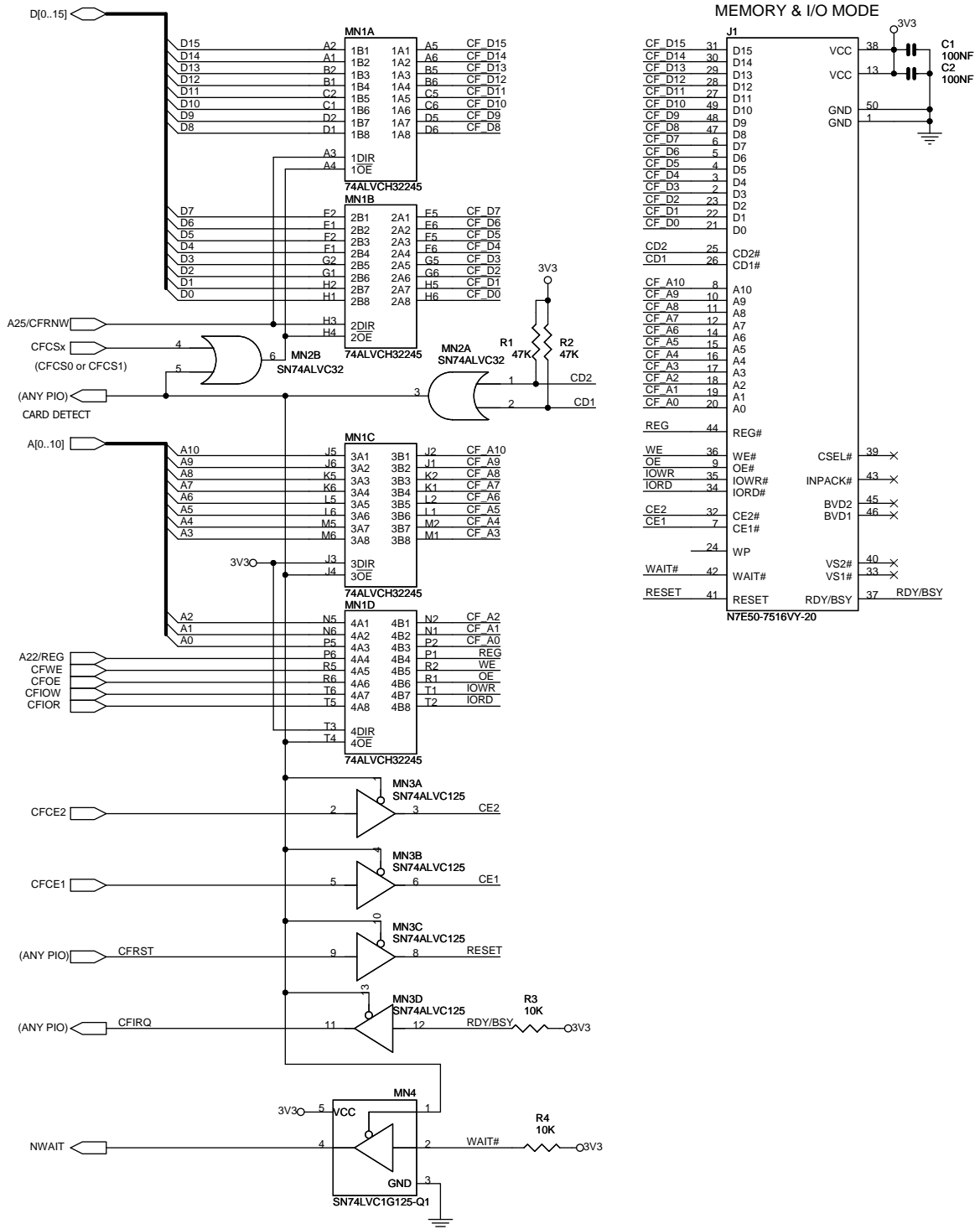
Figure 19-8. Hardware Configuration
