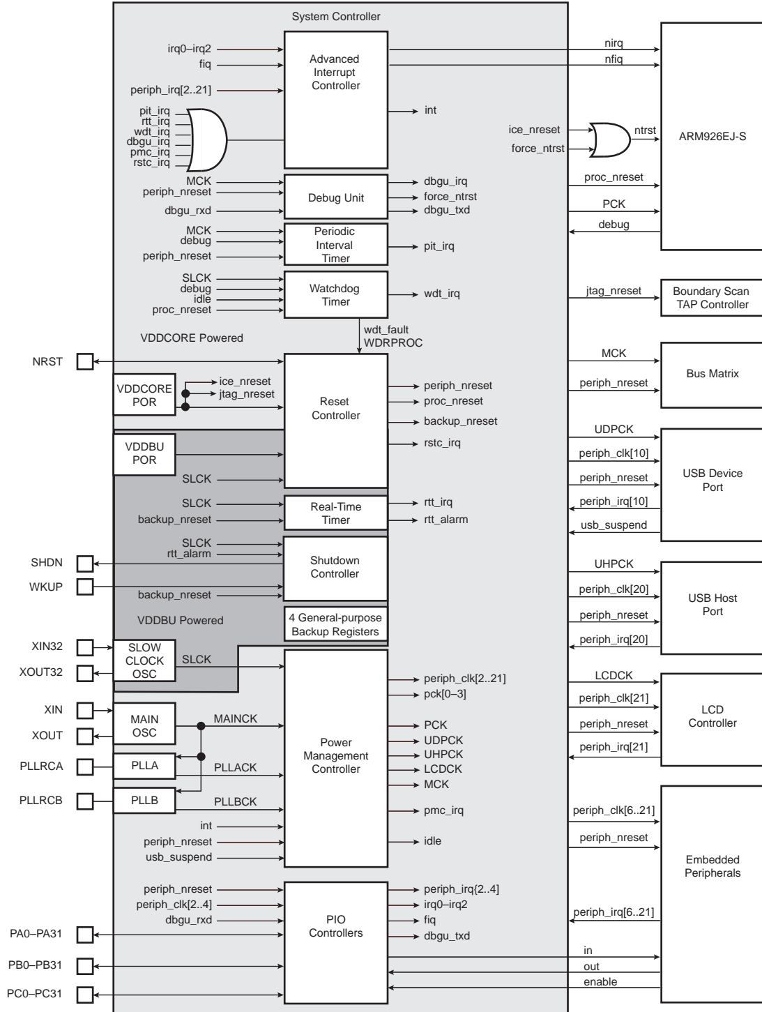
Figure 8-1. System Controller Block Diagram
