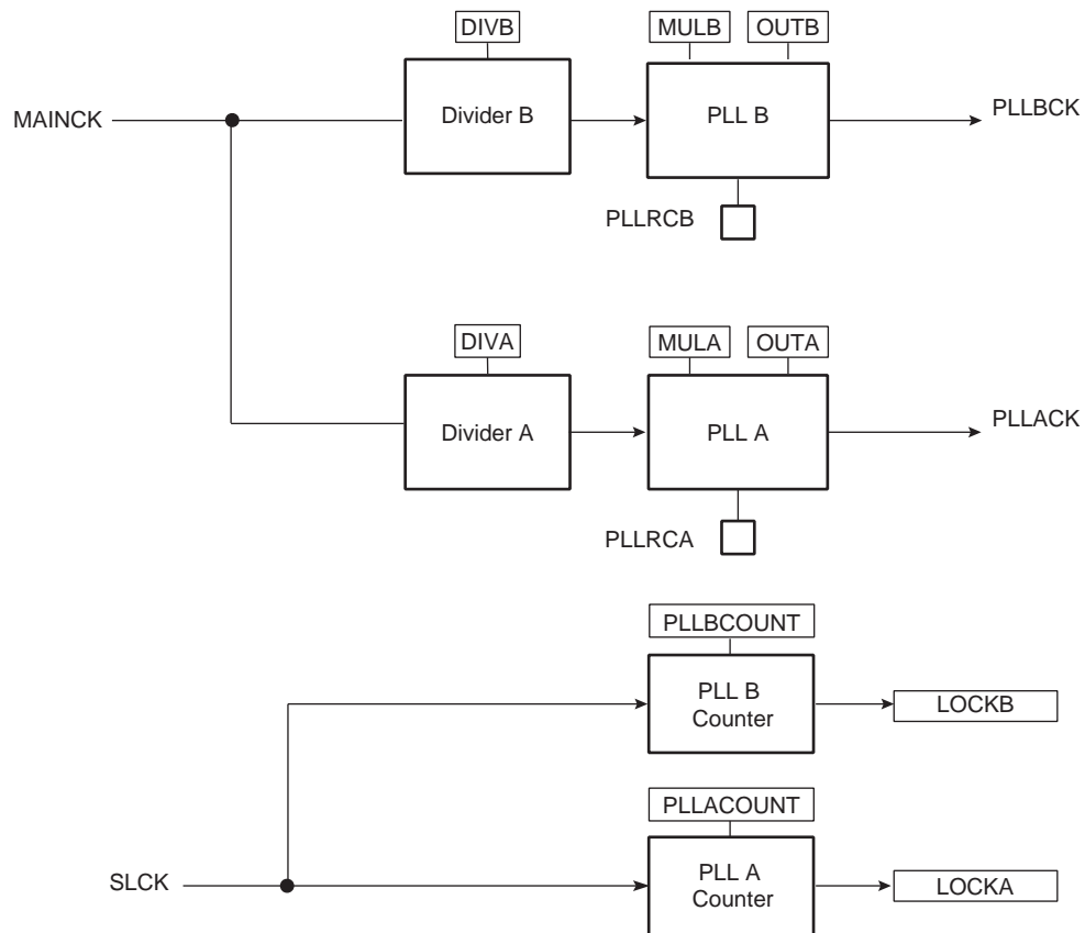
Figure 23-4. Divider and PLL Block Diagram
