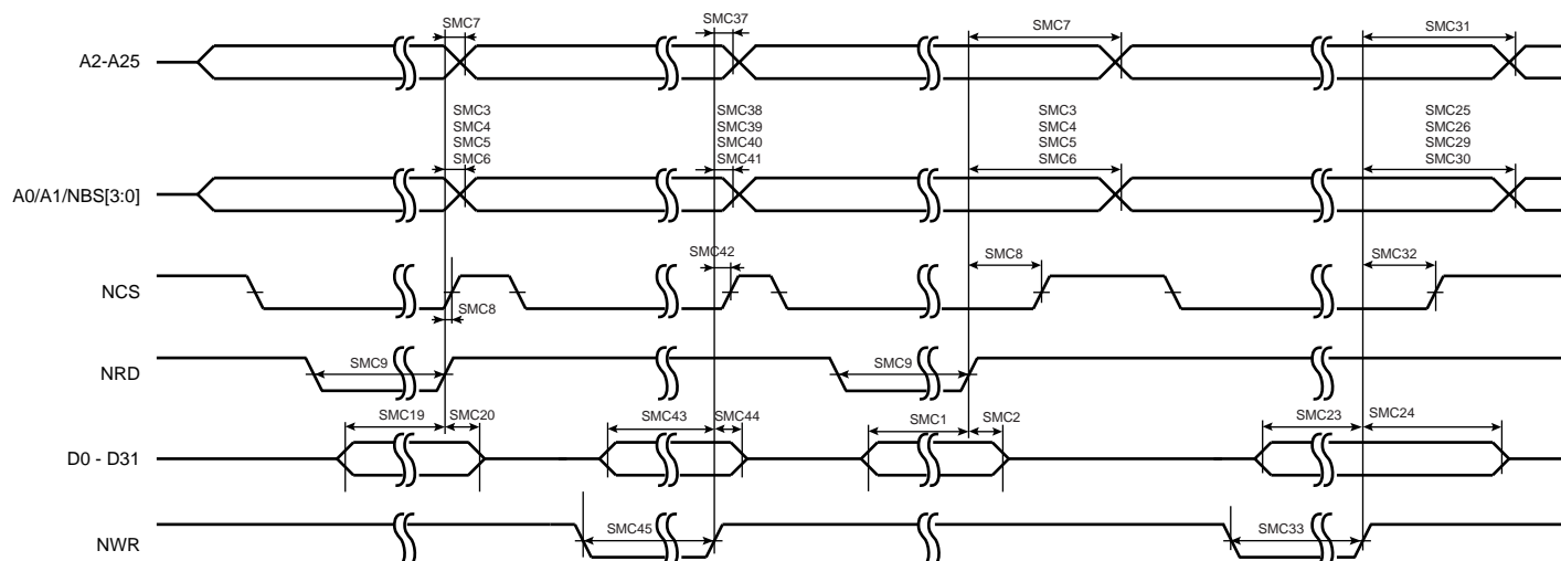
Figure 38-5. SMC Signals for NRD and NWR Controlled Access
