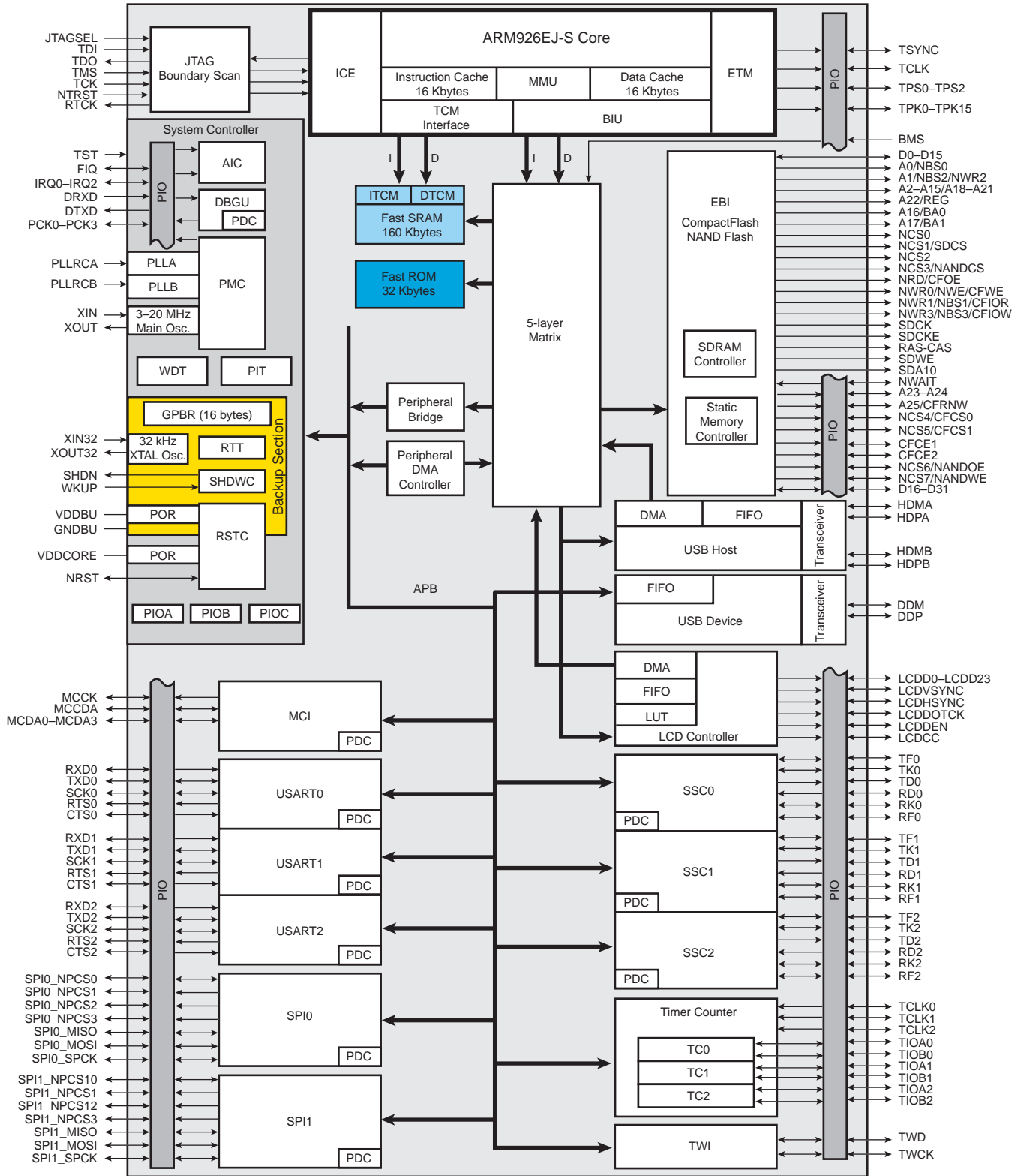
Figure 1-1. SAM9261 Block Diagram
