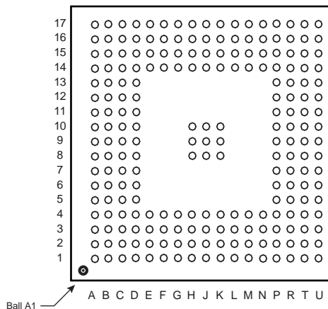
Figure 3-1. 217-ball LFBGA Package Outline (Top View)
