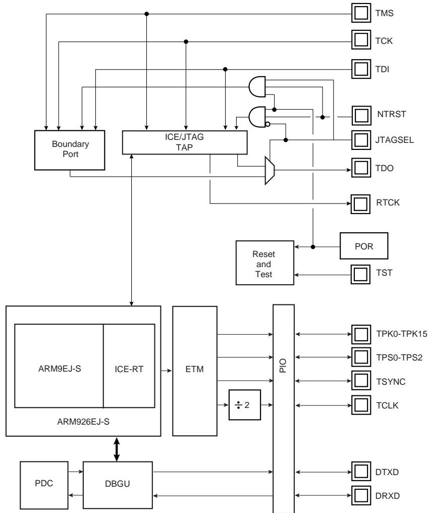
Figure 11-1. Debug and Test Block Diagram
