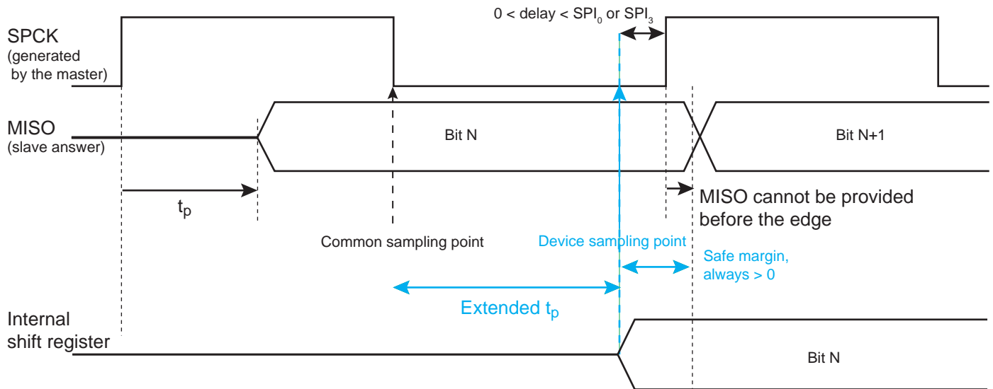
Figure 38-7. MISO Capture in Master Mode
