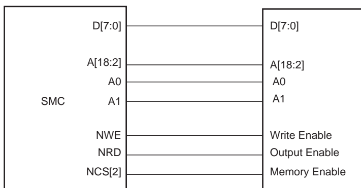
Figure 20-4. Memory Connection for a 16-bit Data Bus
