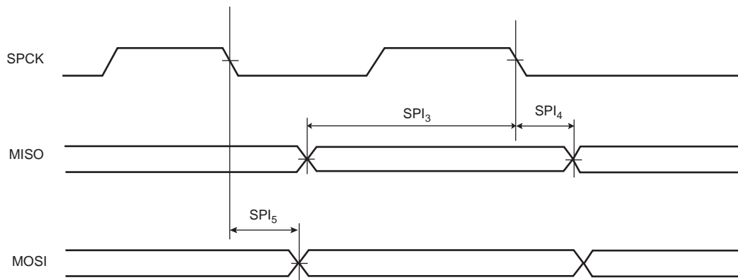
Figure 38-9. SPI Master mode with (CPOL = NCPHA = 0) or (CPOL = NCPHA = 1)
