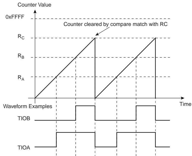
Figure 33-10. WAVSEL = 10 With Trigger
