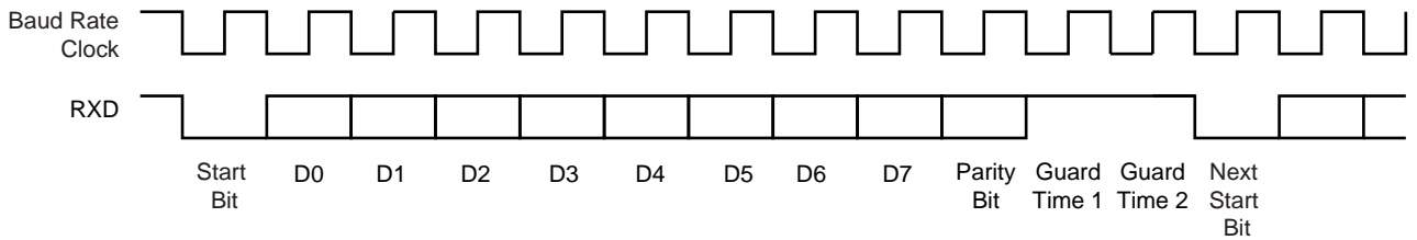
Figure 31-21. T = 0 Protocol without Parity Error
