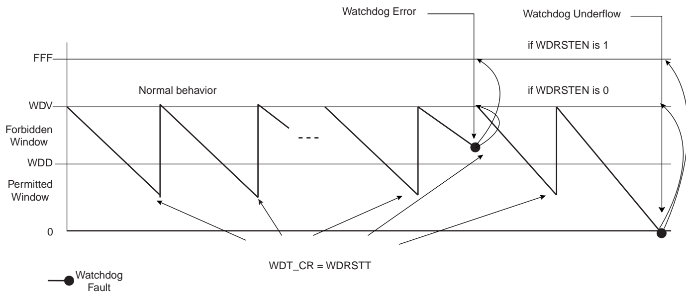
Figure 25-2. Watchdog Behavior
