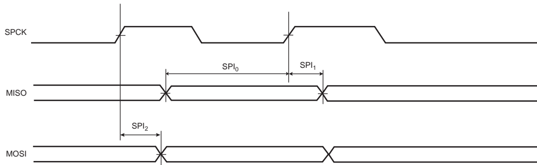
Figure 38-8. SPI Master mode with (CPOL = 0 and NCPHA = 1) or (CPOL = 1 and NCPHA = 0)
