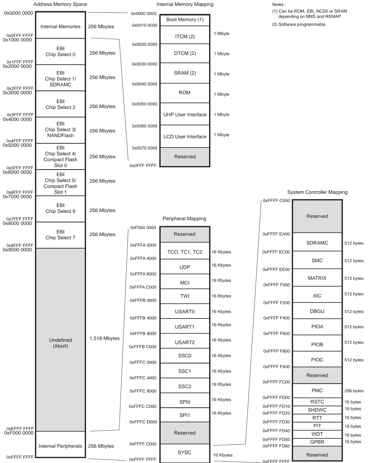
Figure 7-1. SAM9261 Memory Mapping
