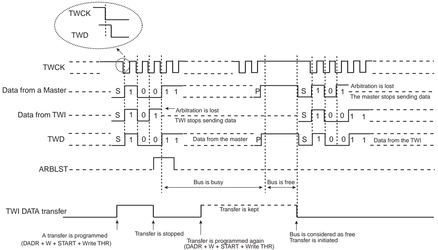
Figure 30-22. Arbitration Cases
