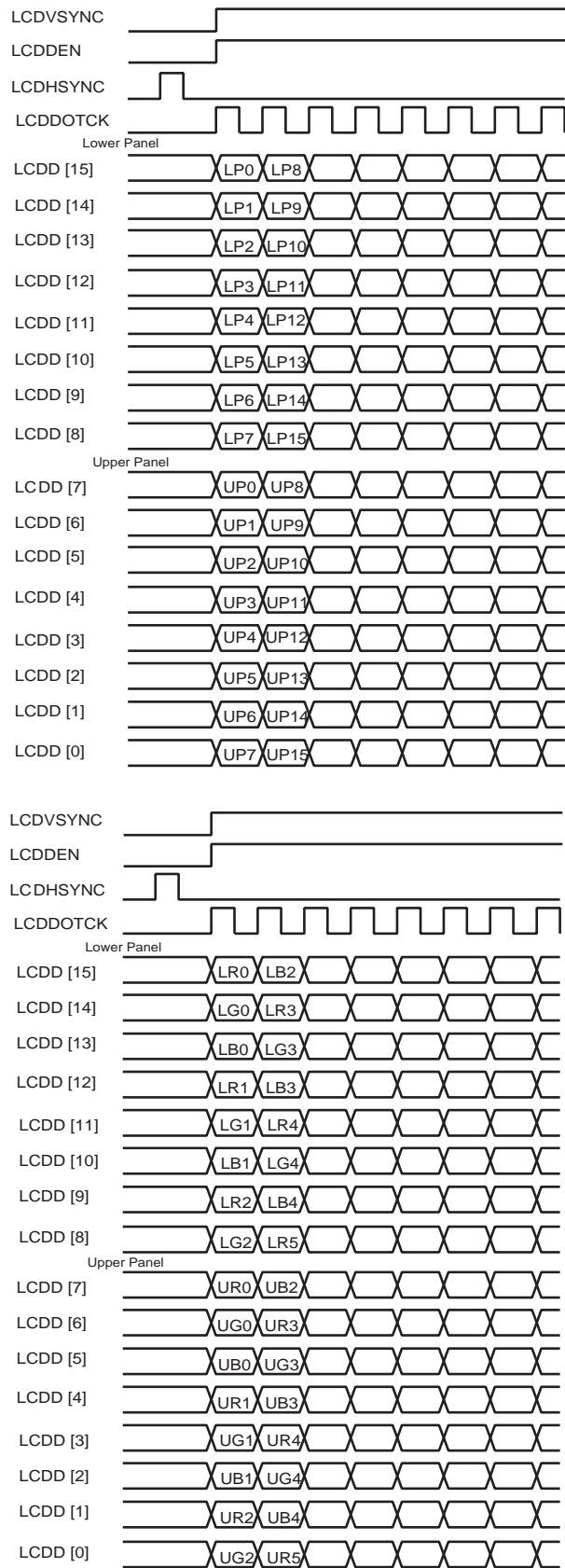
Figure 37-10. Dual Scan Monochrome and Color 16-bit Panel Timing (First Line Expanded View)
