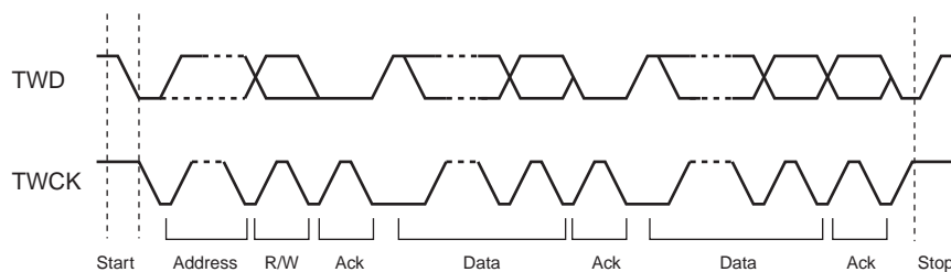
Figure 30-4. Transfer Format
