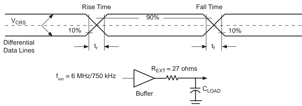
Figure 38-13. USB Data Signal Timing Diagram
