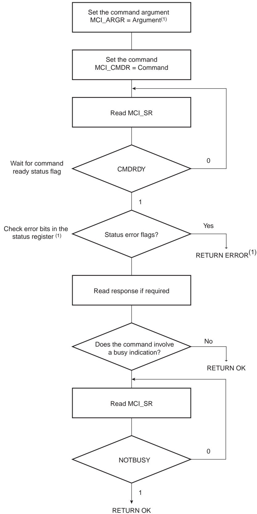
Figure 34-7. Command/Response Functional Flow Diagram
