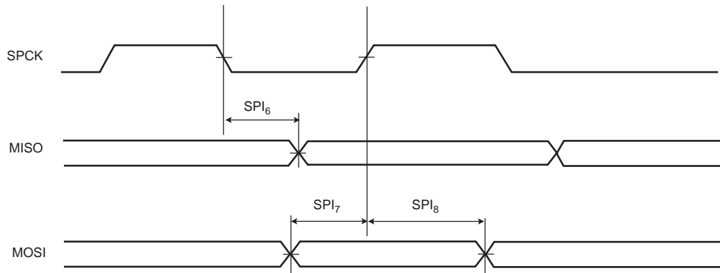
Figure 38-10. SPI Slave mode with (CPOL = 0 and NCPHA = 1) or (CPOL = 1 and NCPHA = 0)
