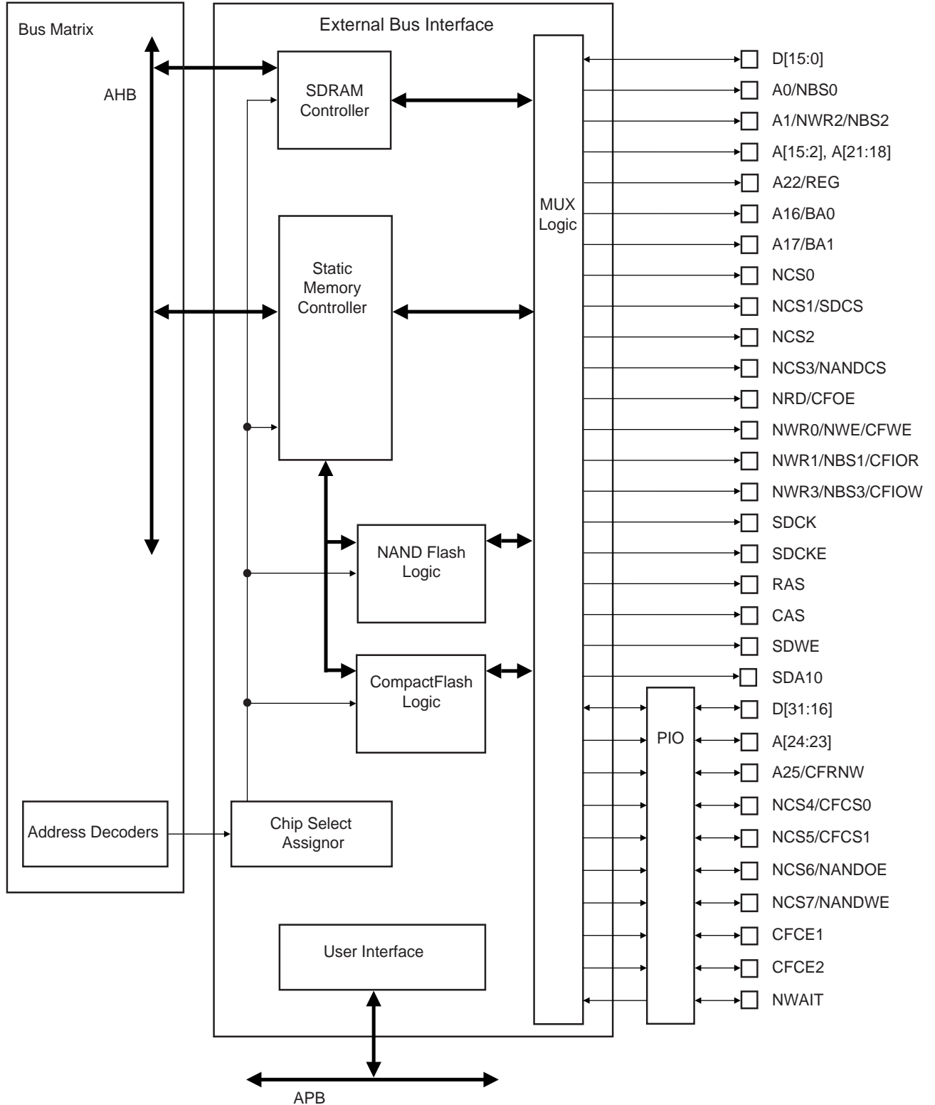
Figure 19-1. Organization of the External Bus Interface
