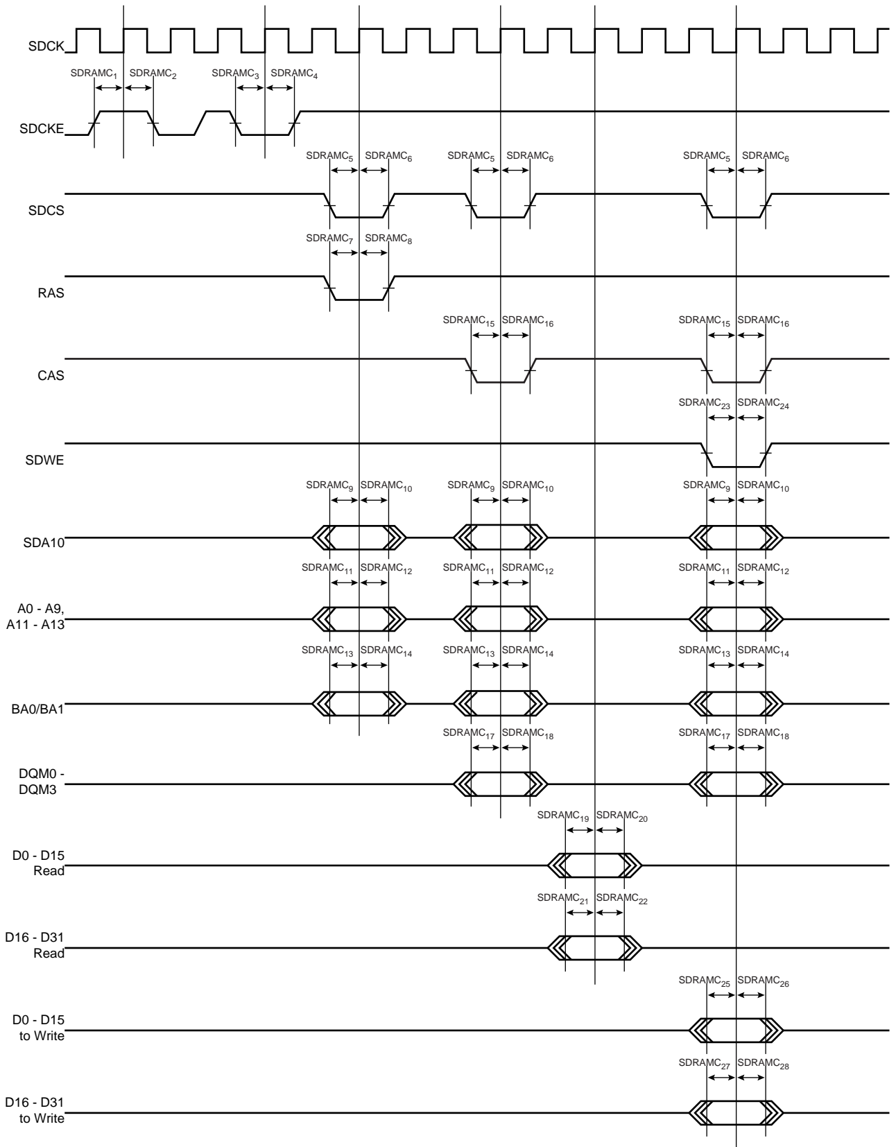
Figure 38-6. SDRAM Signals Relative to SDCK
