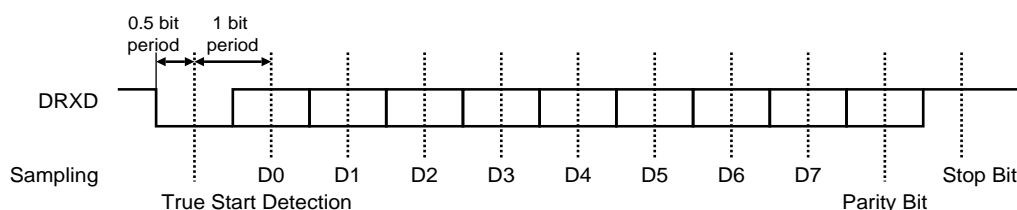
Figure 27-5. Character Reception
