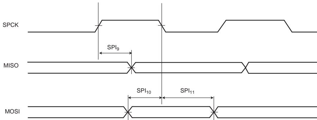
Figure 38-11. SPI Slave mode with (CPOL = NCPHA = 0) or (CPOL = NCPHA = 1)
