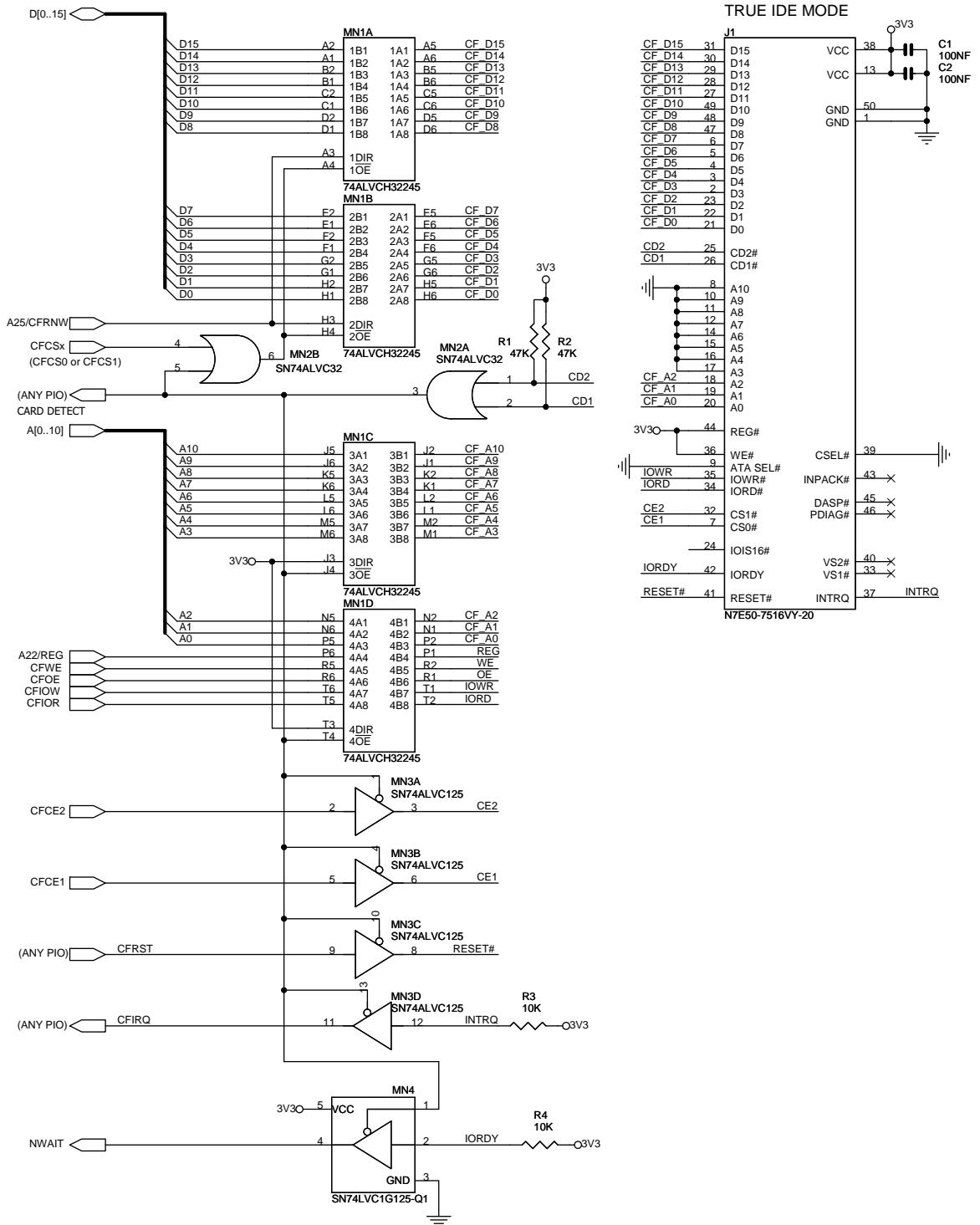
Figure 19-9. Hardware Configuration
