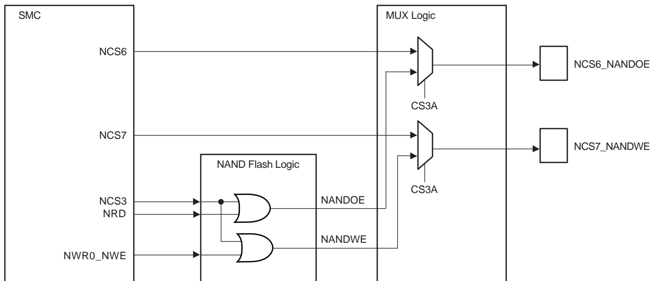
Figure 19-6. NAND Flash Signal Multiplexing on EBI Pins
