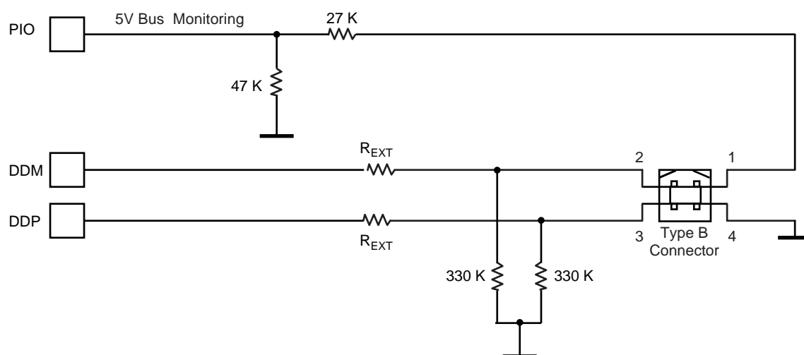
Figure 36-2. Board Schematic to Interface Device Peripheral
