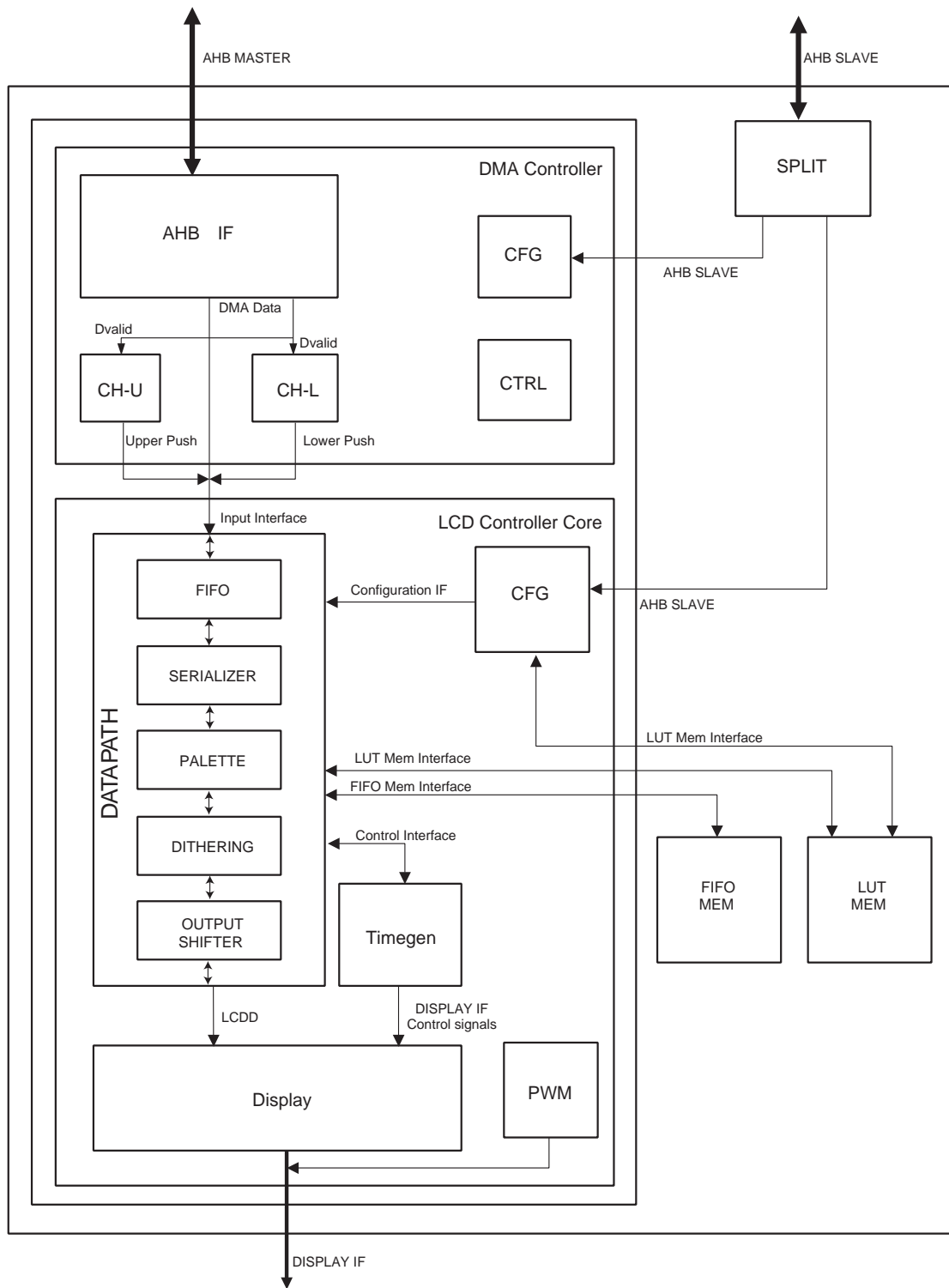
Figure 37-1. LCD Macrocell Block Diagram
