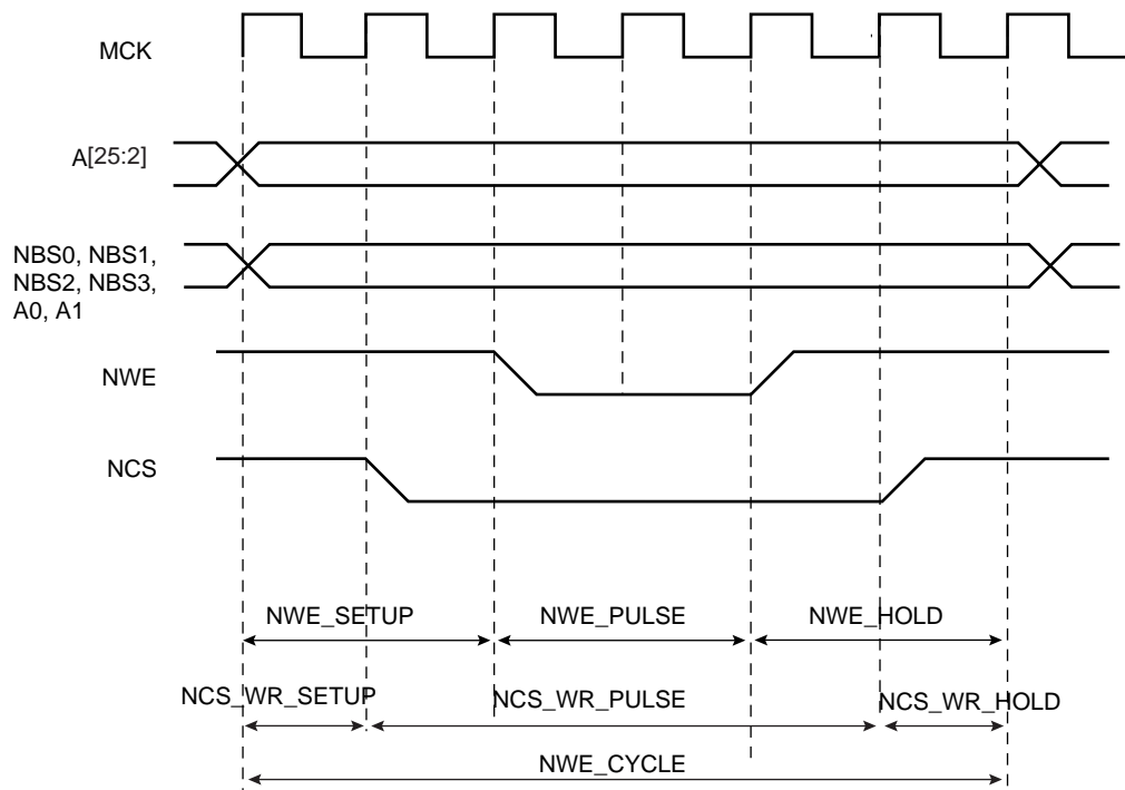
Figure 20-12. Write Cycle
