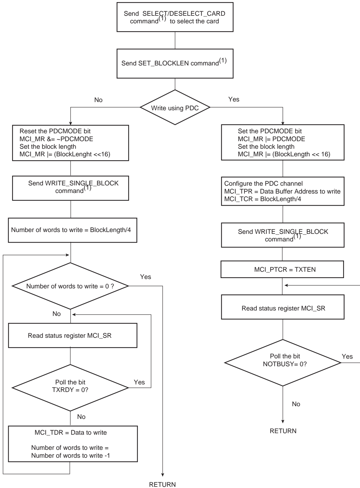
Figure 34-9. Write Functional Flow Diagram
