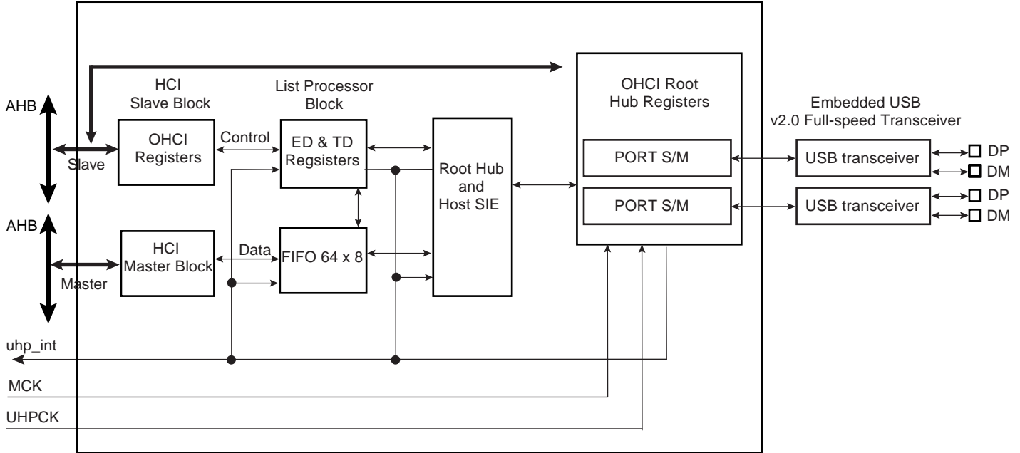
Figure 35-1. Block Diagram
