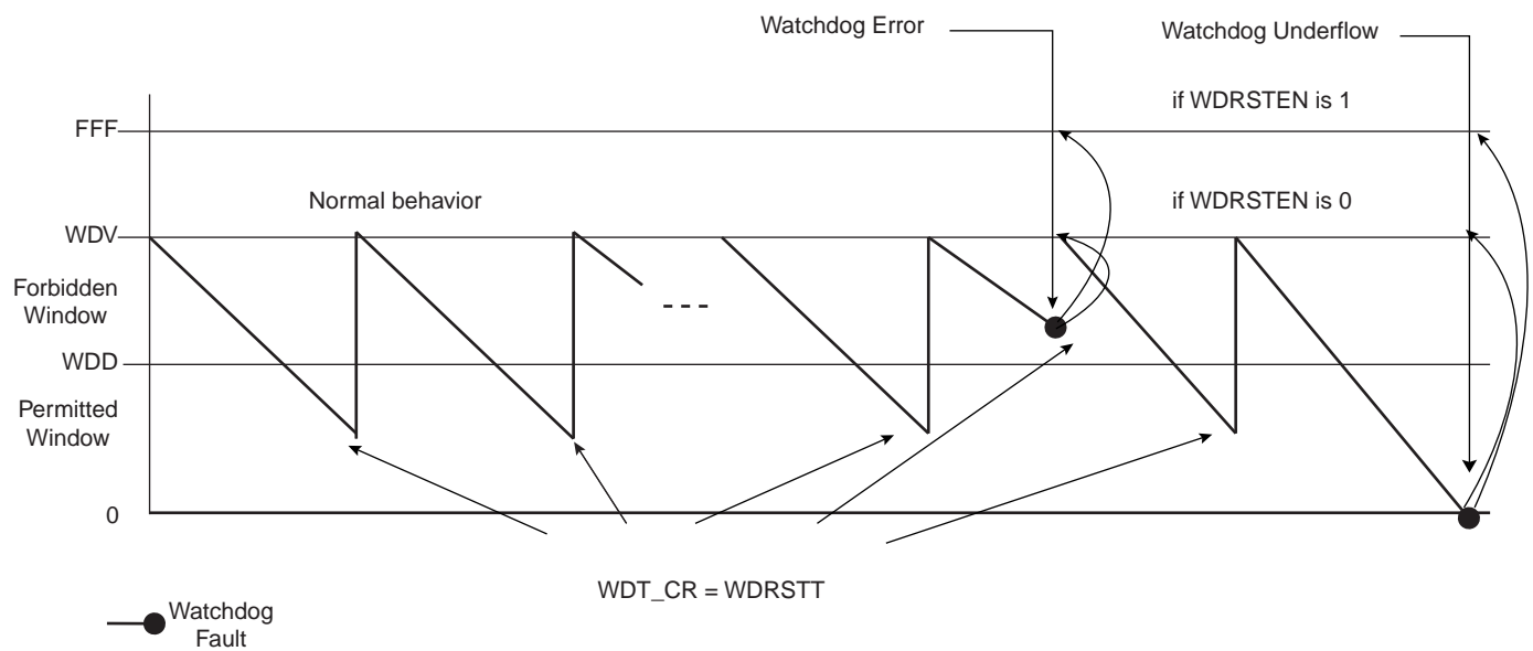
Figure 25-2. Watchdog Behavior
