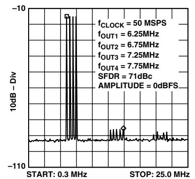
Figure 38. Four-Tone SFDR
