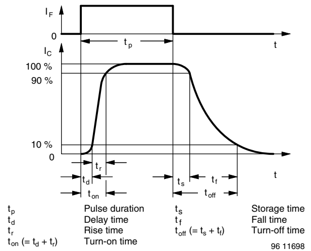
Fig. 3 - Switching Times
