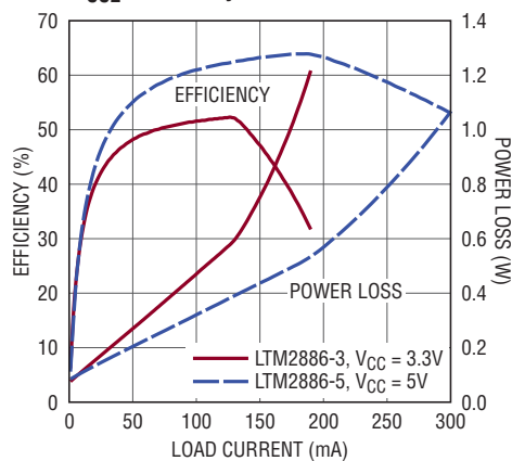
V_{CC2} Efficiency
