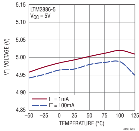
V^- Load Regulation vs Temperature
