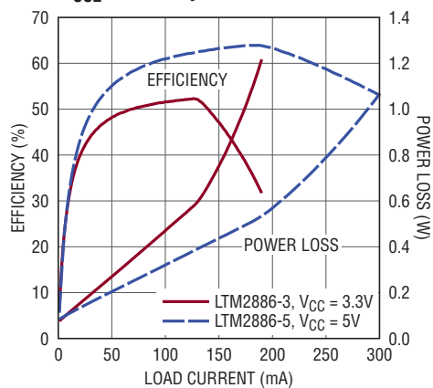
V_{CC2} Efficiency
