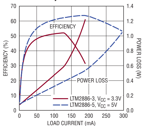
V^+ Efficiency
