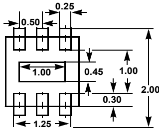
LAND PATTERN \triangle 6
