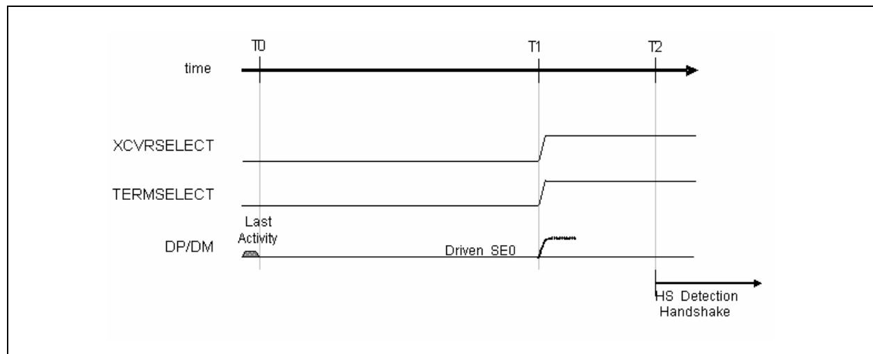
Figure 7.1 Reset Timing Behavior (HS Mode)
