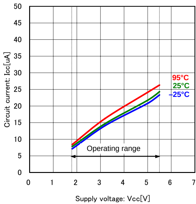
Fig.3 Circuit current
