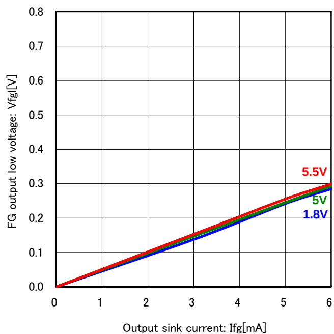
Fig.10 FG output low voltage ( T_a=25^{\circ}C )
