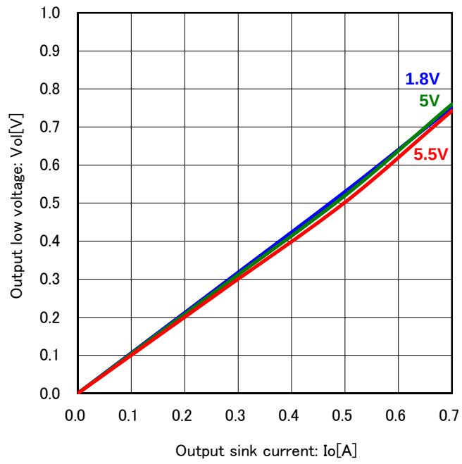
Fig.8 Output voltage ( T_a=25^{\circ}C )
