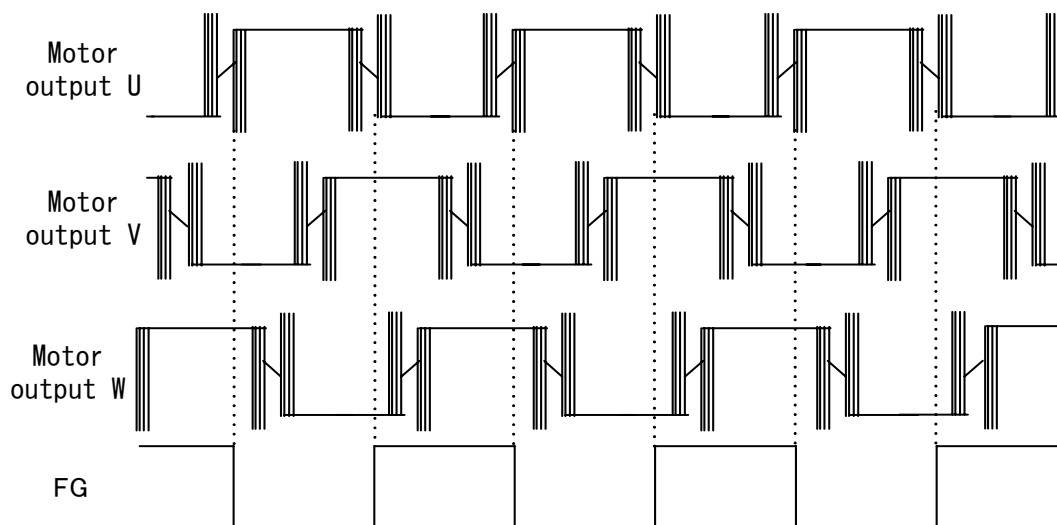
Fig.13 Motor Output , FG signal
