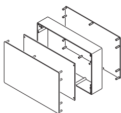
Explosion drawing
