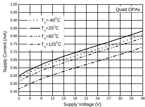
Supply Current vs. Supply Voltage (LM2902/LM2902A)
